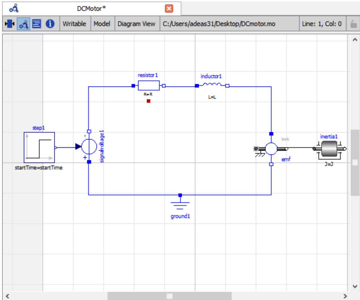
Figure 2.9: Model Widget showing the Diagram View.
