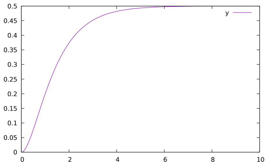
Figure 11.11: Characteristic equation with real negative roots.
