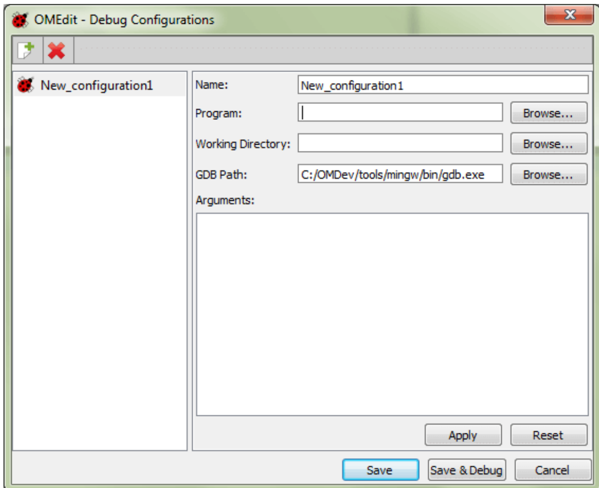
Figure 5.4: Debug Configurations.
