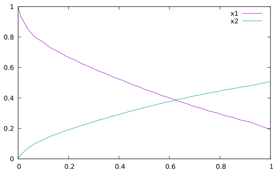
Figure 12.2: Optimization results for Batch Reactor model – state variables.
