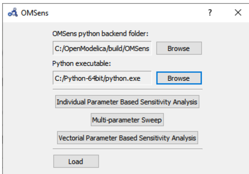
Figure 13.3: OMSens window.
