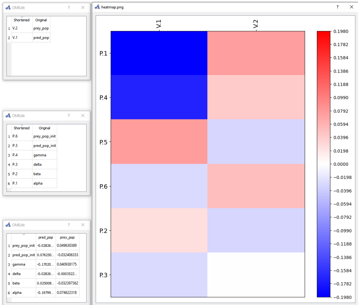
Figure 13.9: Individual sensitivity analysis heatmap.
