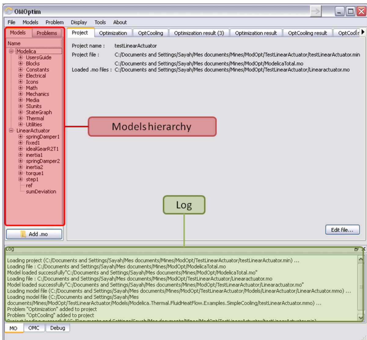
Figure 12.3: OMOptim window after having loaded model.
