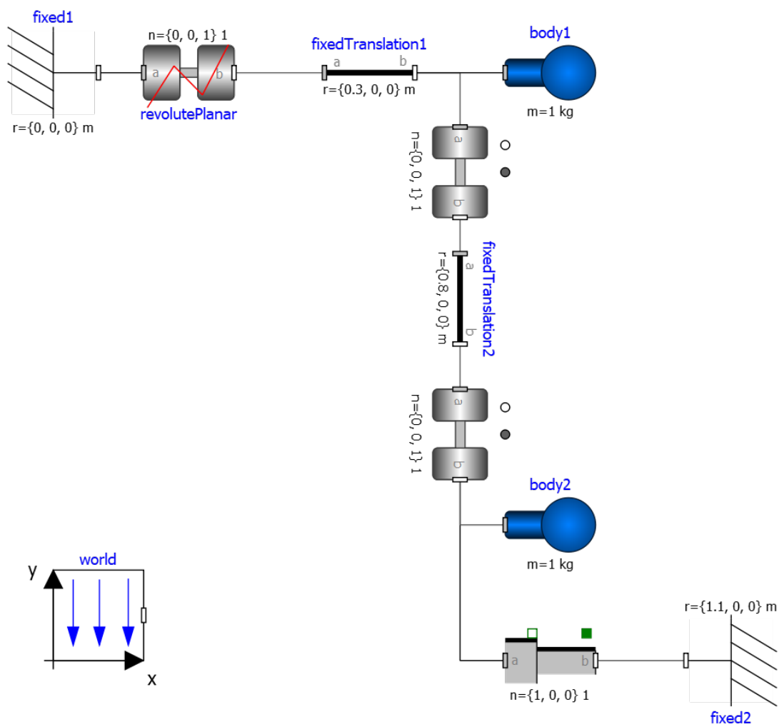
Figure 4.1: piston.mo
