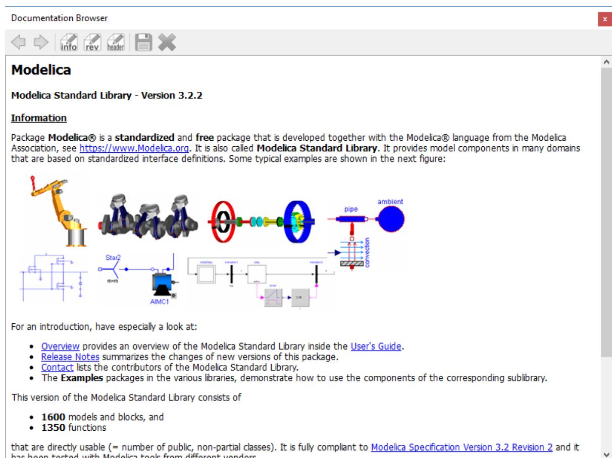
Figure 2.3: Documentation Browser.
