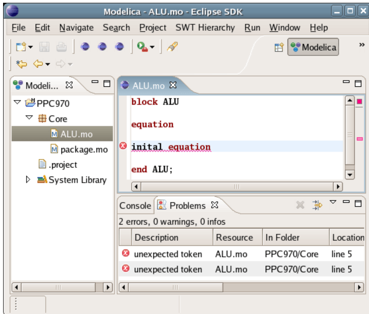
Figure 14.10: Syntax checking.
