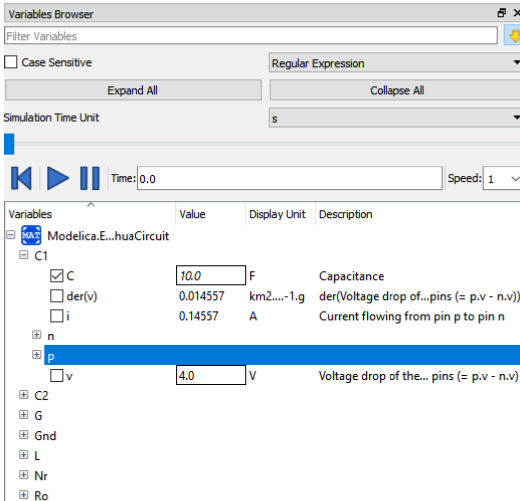
Figure 2.5: Variables Browser.
