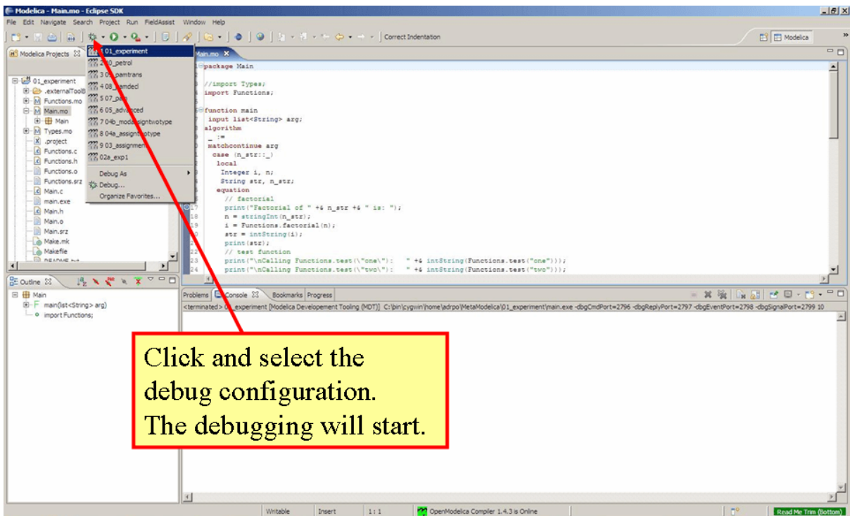
Figure 15.5: Starting the debugging session.
