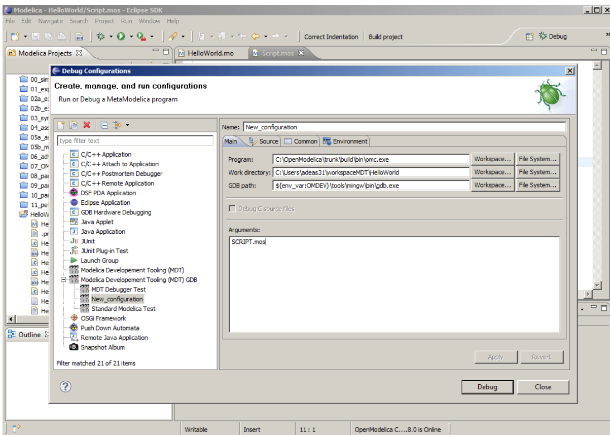
Figure 15.3: Creating the Debug Configuration.
