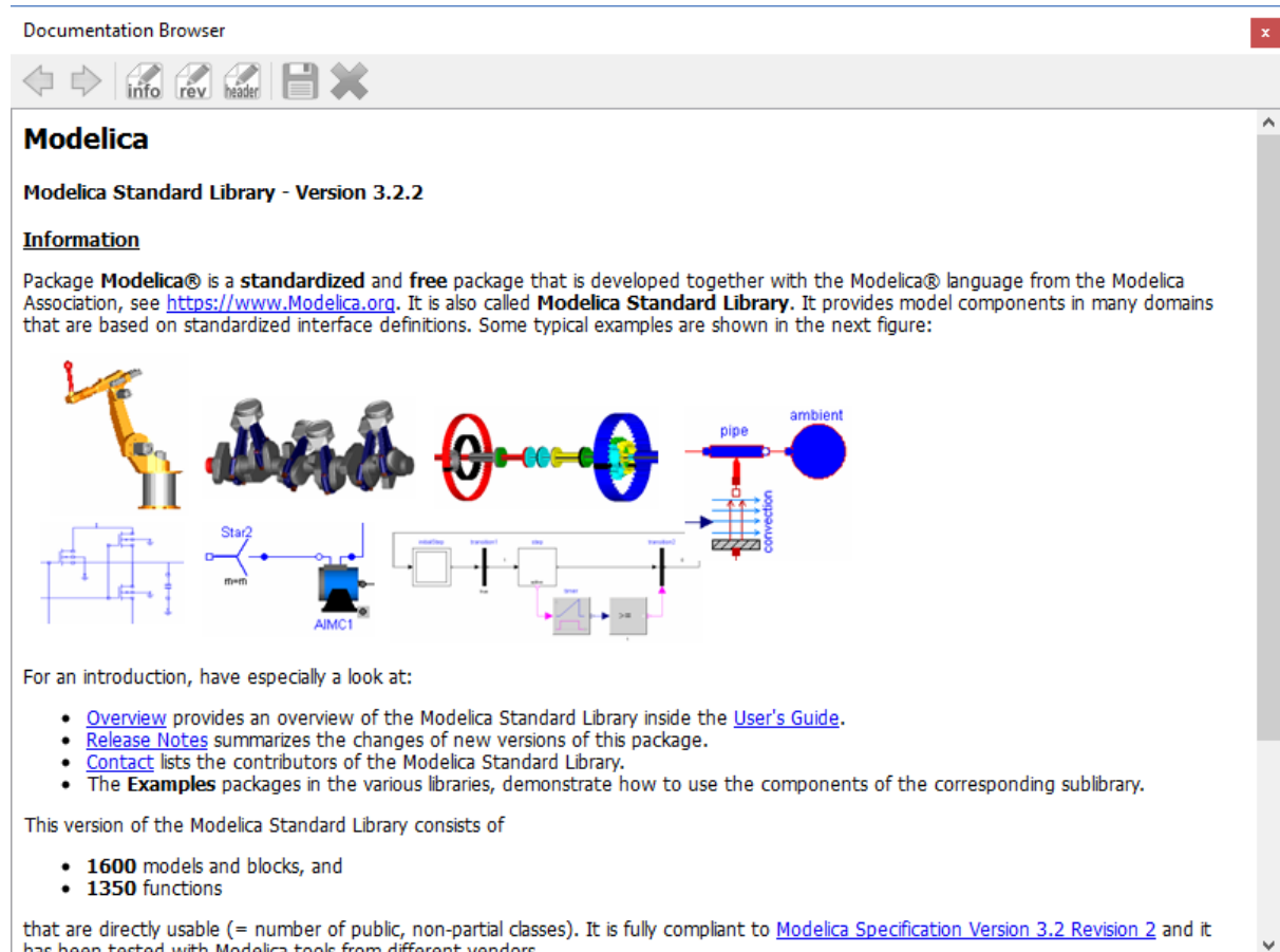
Figure 3.3: Documentation Browser.
