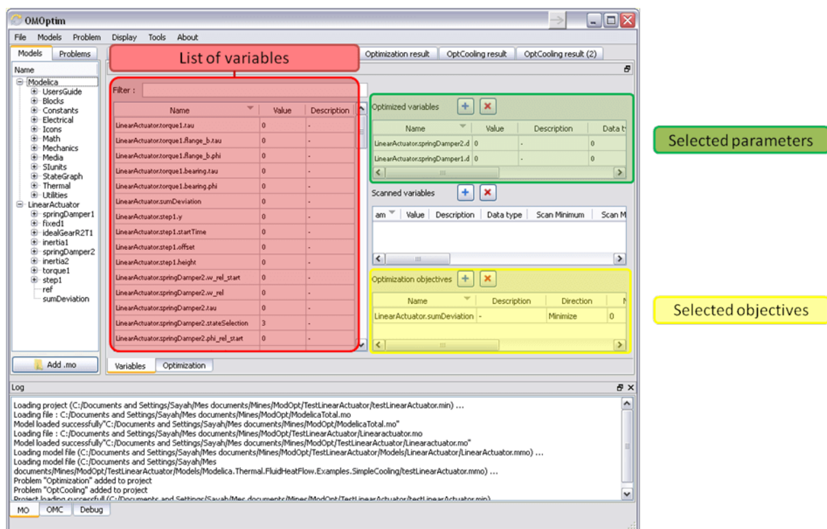
Figure 15.4: Forms for defining a new optimization problem.
