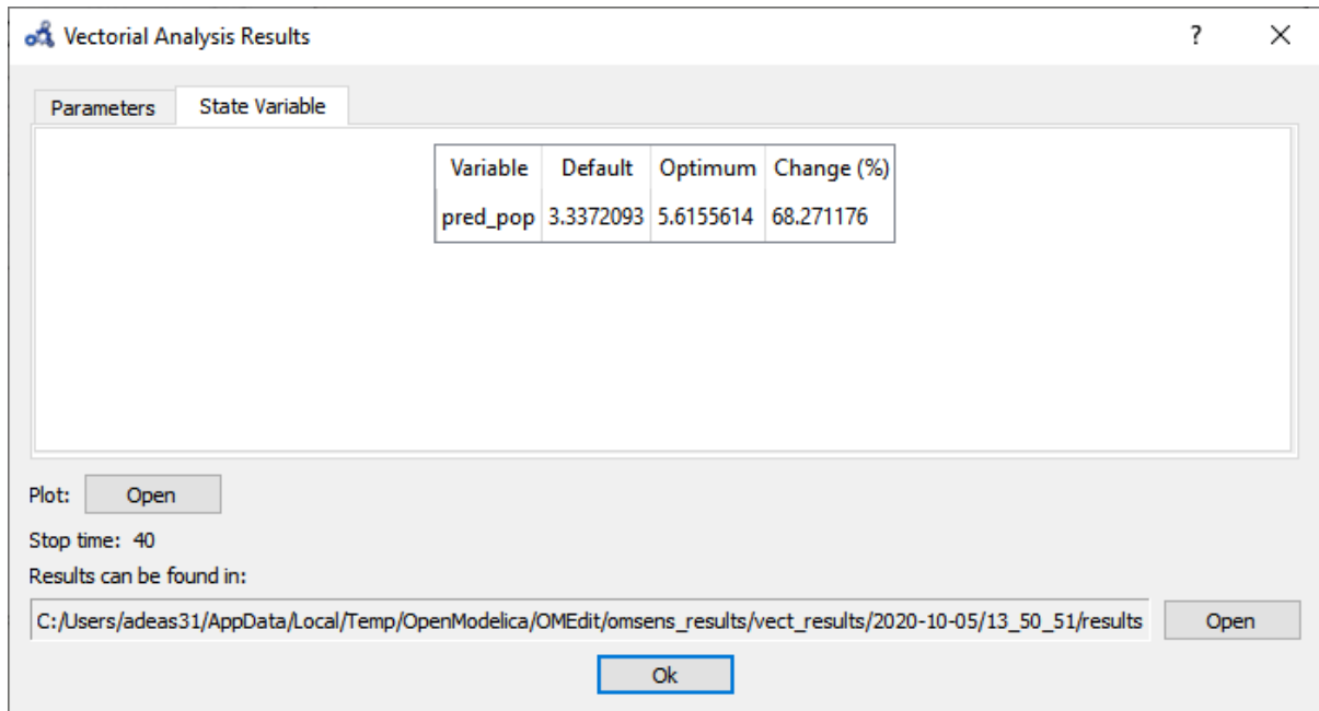
Figure 16.20: Vectorial sensitivity analysis state variables.
