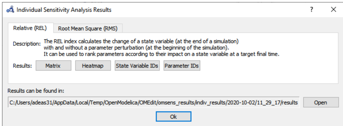
Figure 16.8: Individual sensitivity analysis results.
