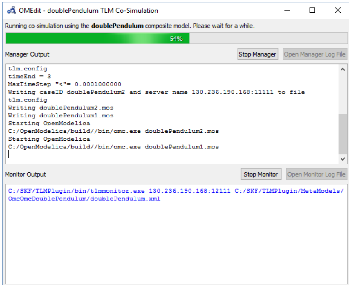
Figure 10.5: TLM Co-Simulation Progress.
