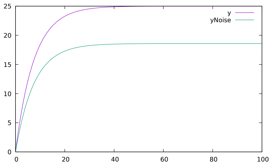
Figure 14.8: Open loop control example.
