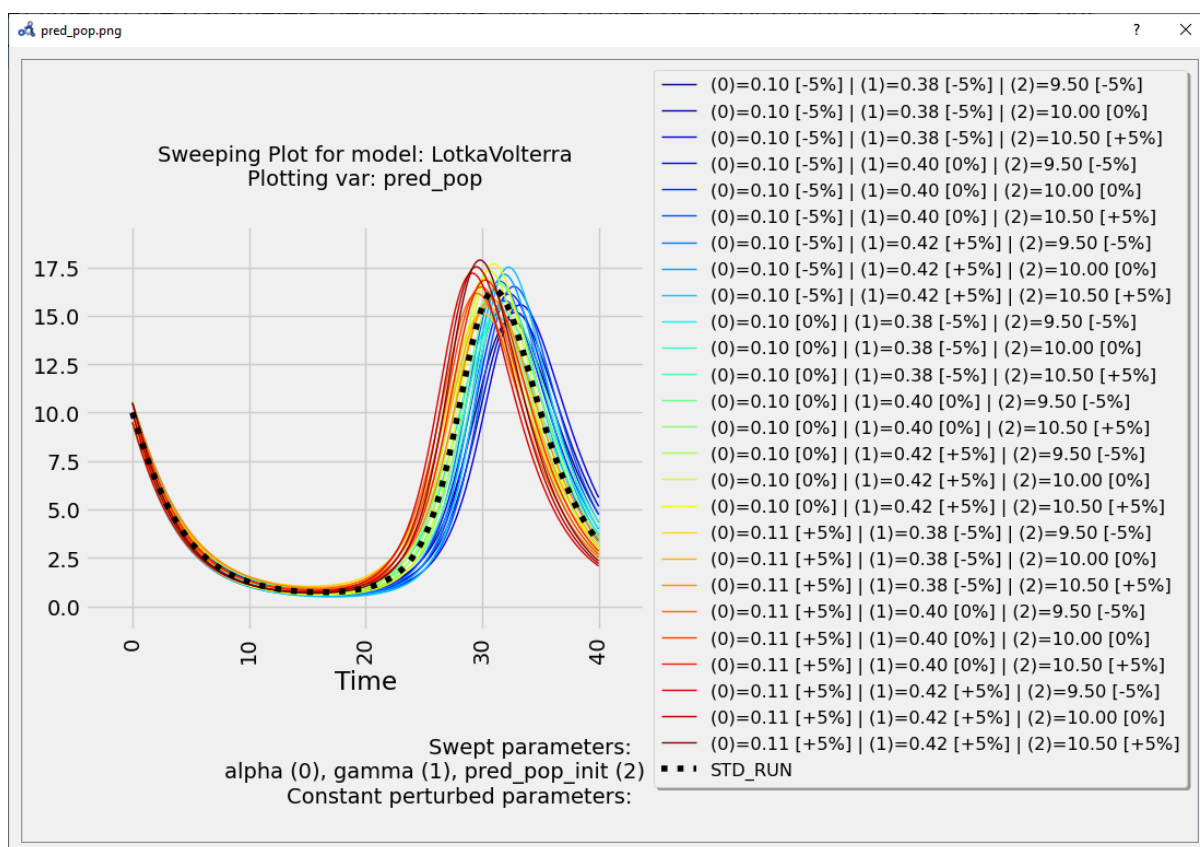
Figure 16.12: Multi-parameter sweep plot.
