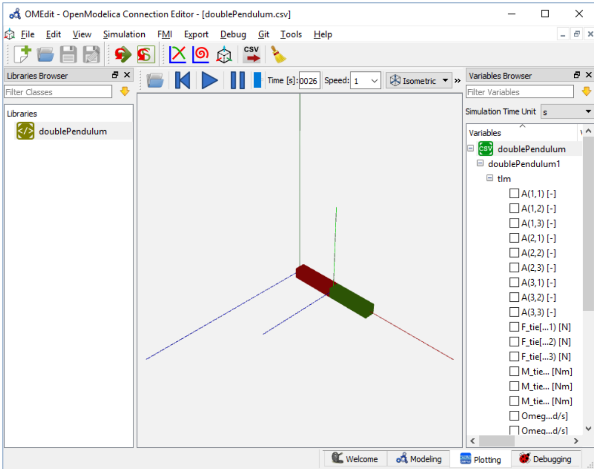
Figure 10.7: TLM Co-Simulation Visualization.
