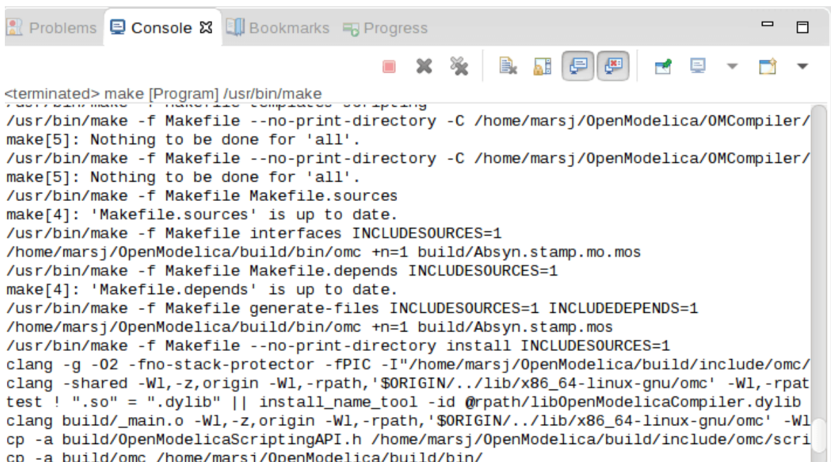
Figure 18.6: Eclipse - building a project, resulting log.
