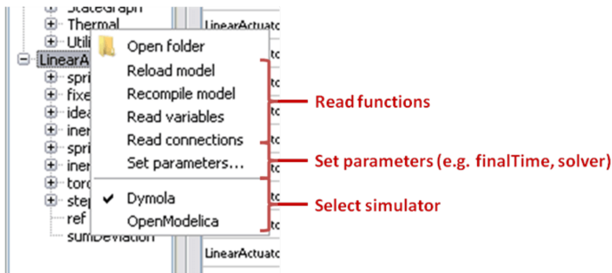
Figure 15.5: Selecting read variables, set parameters, and selecting simulator.
