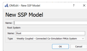
Figure 11.4: OMEdit: New SSP Model Dialog
