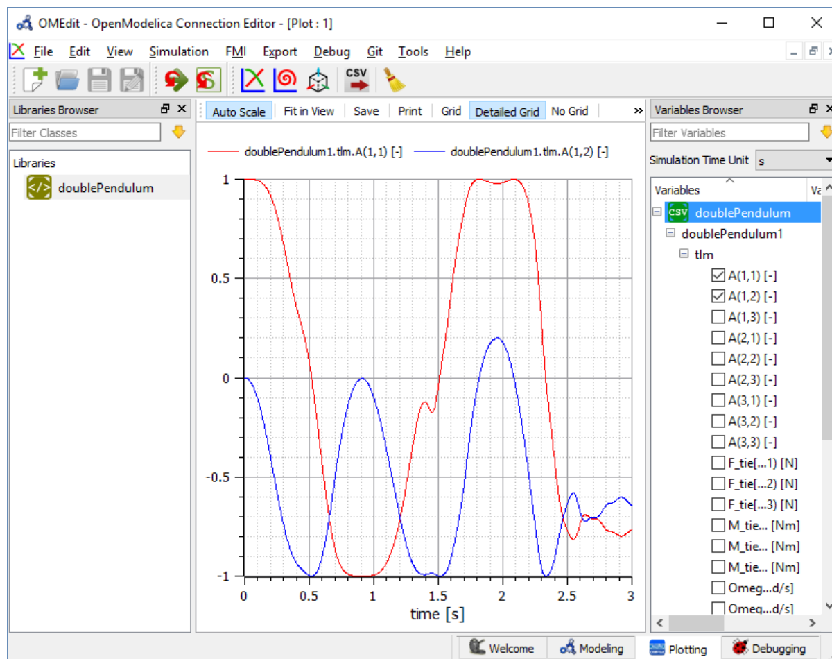
Figure 10.6: TLM Co-Simulation Results Plotting.
