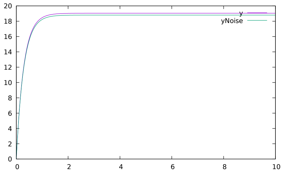
Figure 14.9: Closed loop control example.
