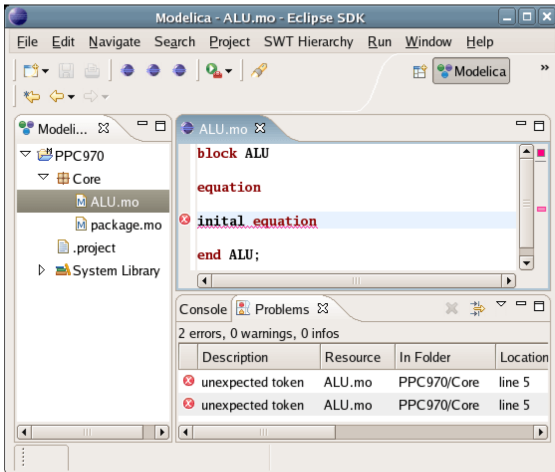
Figure 18.10: Syntax checking.
