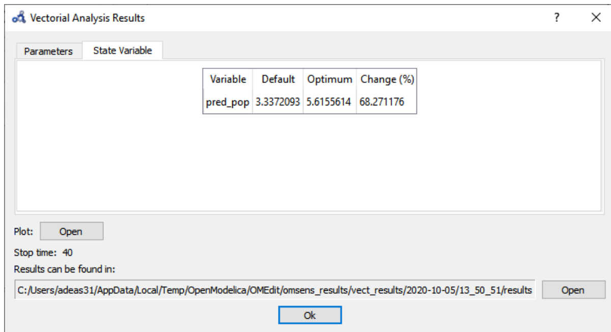
Figure 16.16: Vectorial sensitivity analysis state variables.
