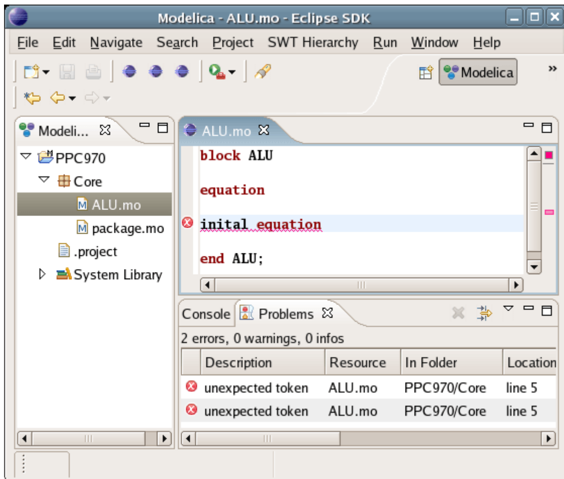
Figure 19.10: Syntax checking.
