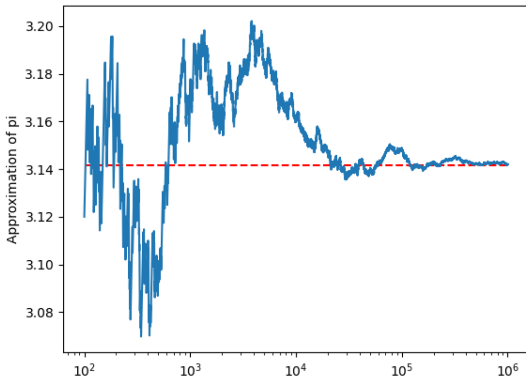
Figure 9.1: Results of the above batch simulation which approximates the value of pi
