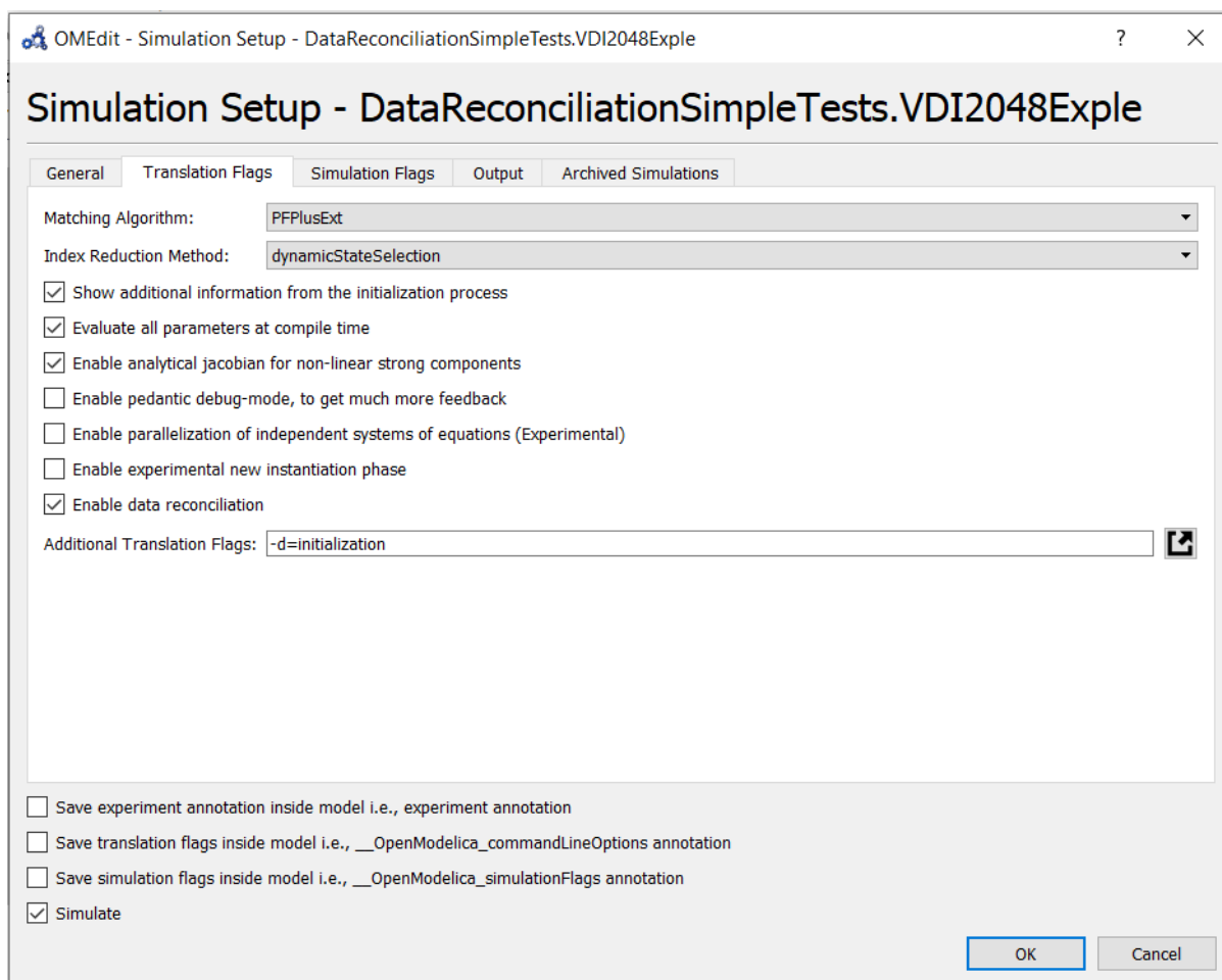
Figure 30.2: Setting DataReconciliation TraslationFlag
