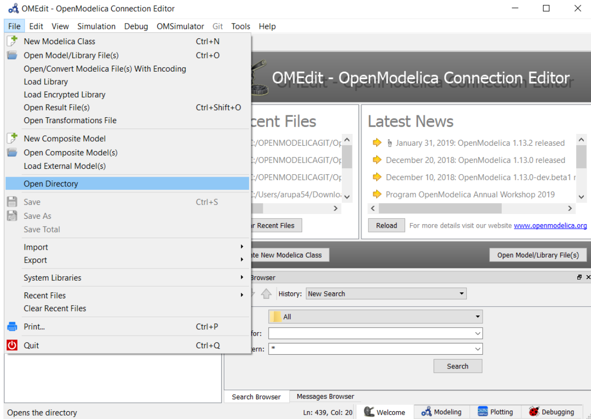
Figure 2.16: open-directory
