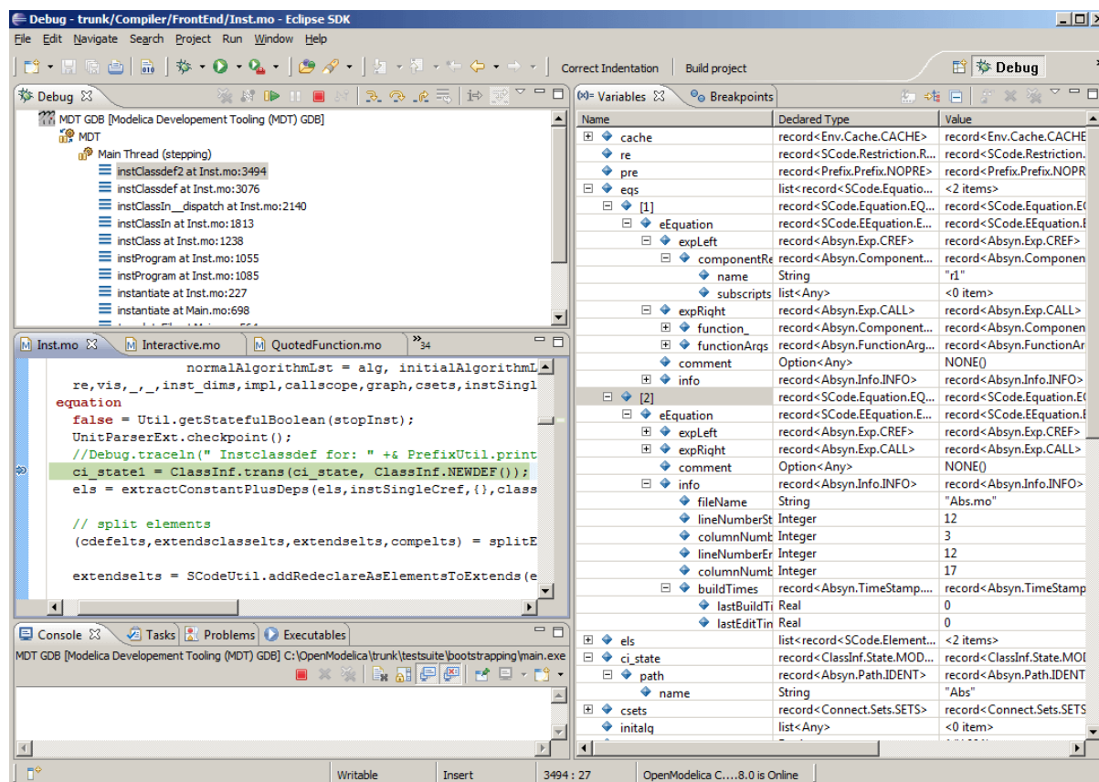
Figure 16.1: Debugging functionality.
