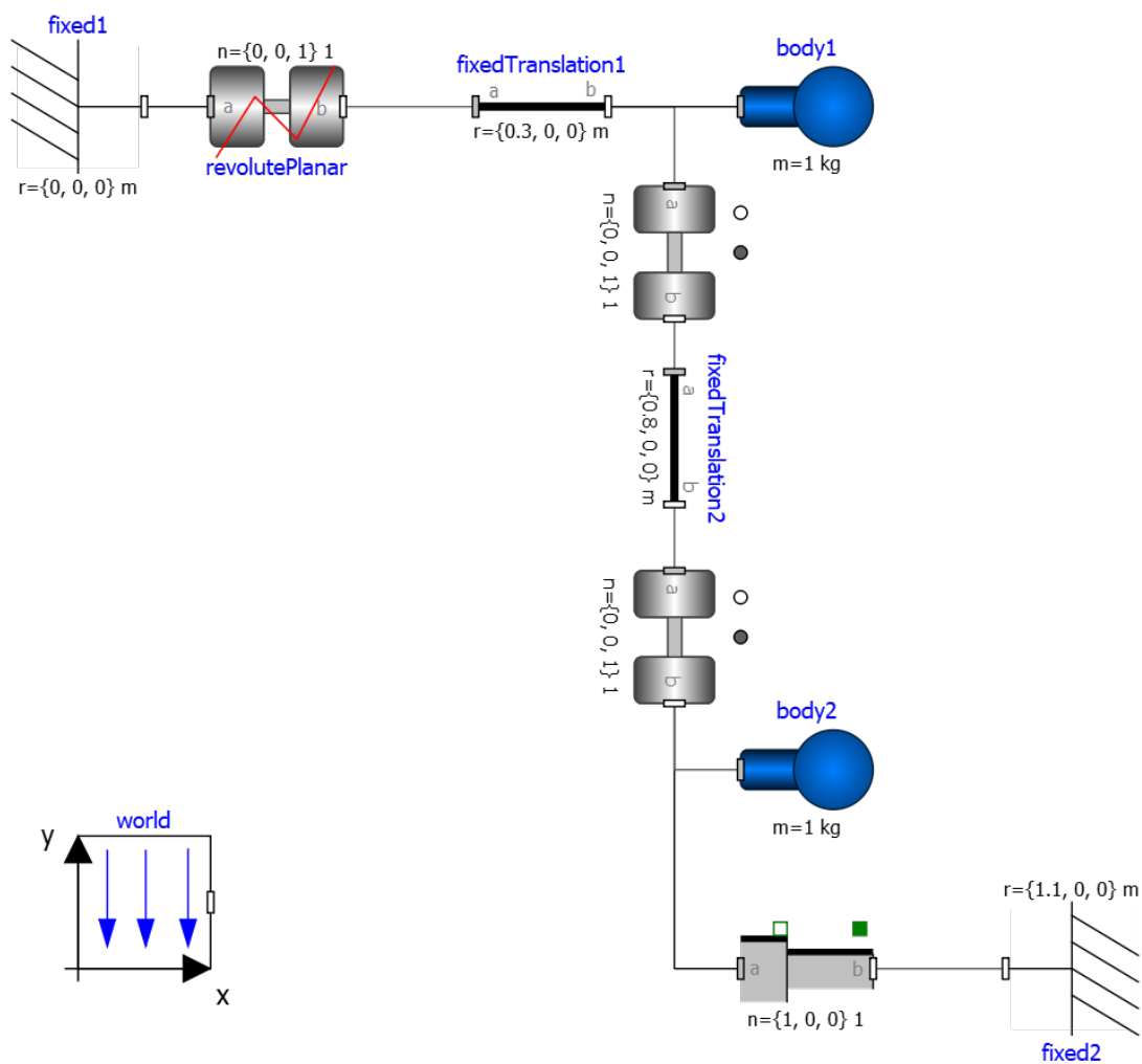
Figure 4.1: piston.mo
