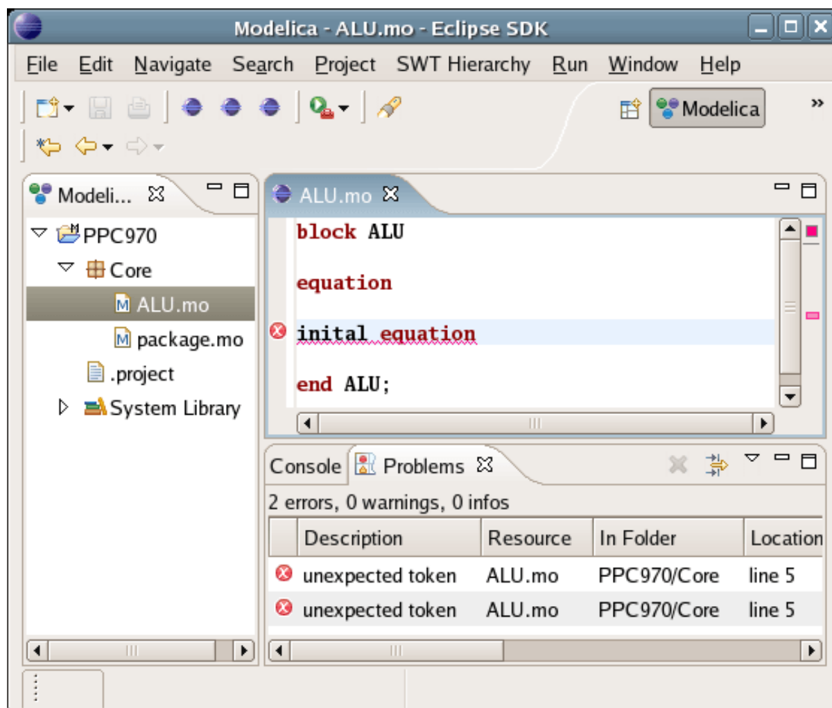
Figure 15.10: Syntax checking.
