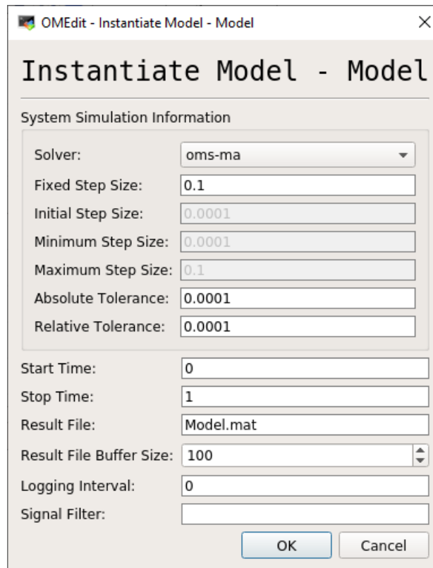
Figure 8.9: OMEdit: Instantiate Model Dialog
