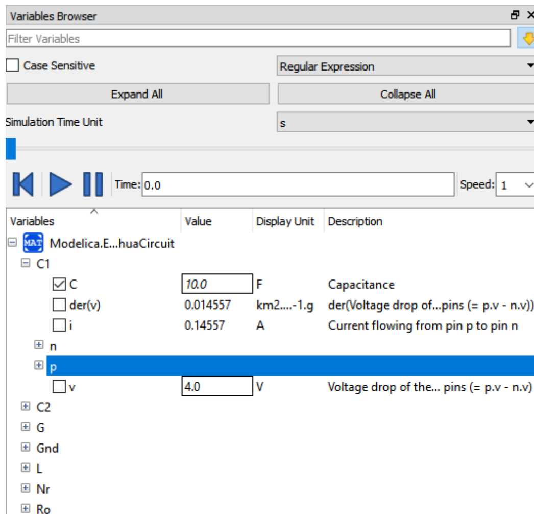
Figure 2.5: Variables Browser.
