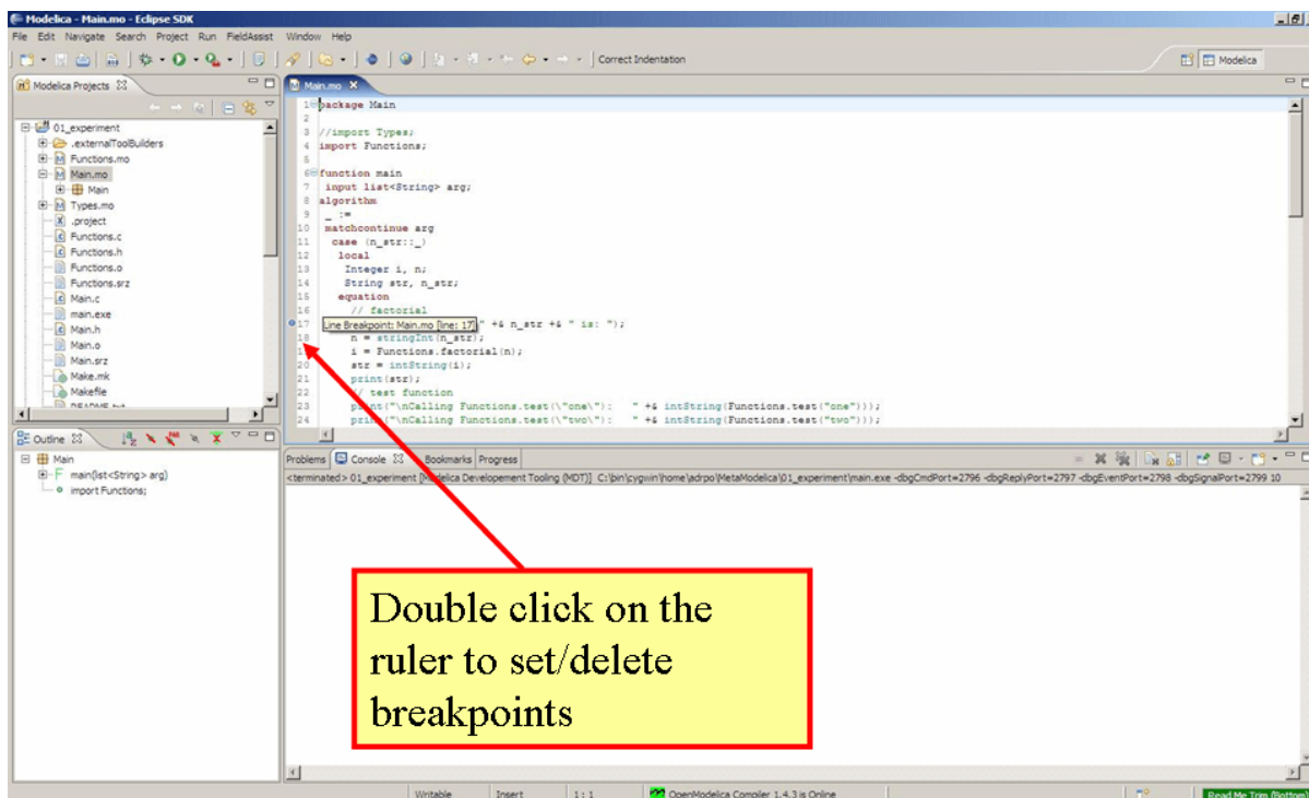
Figure 17.4: Setting/deleting breakpoints.
