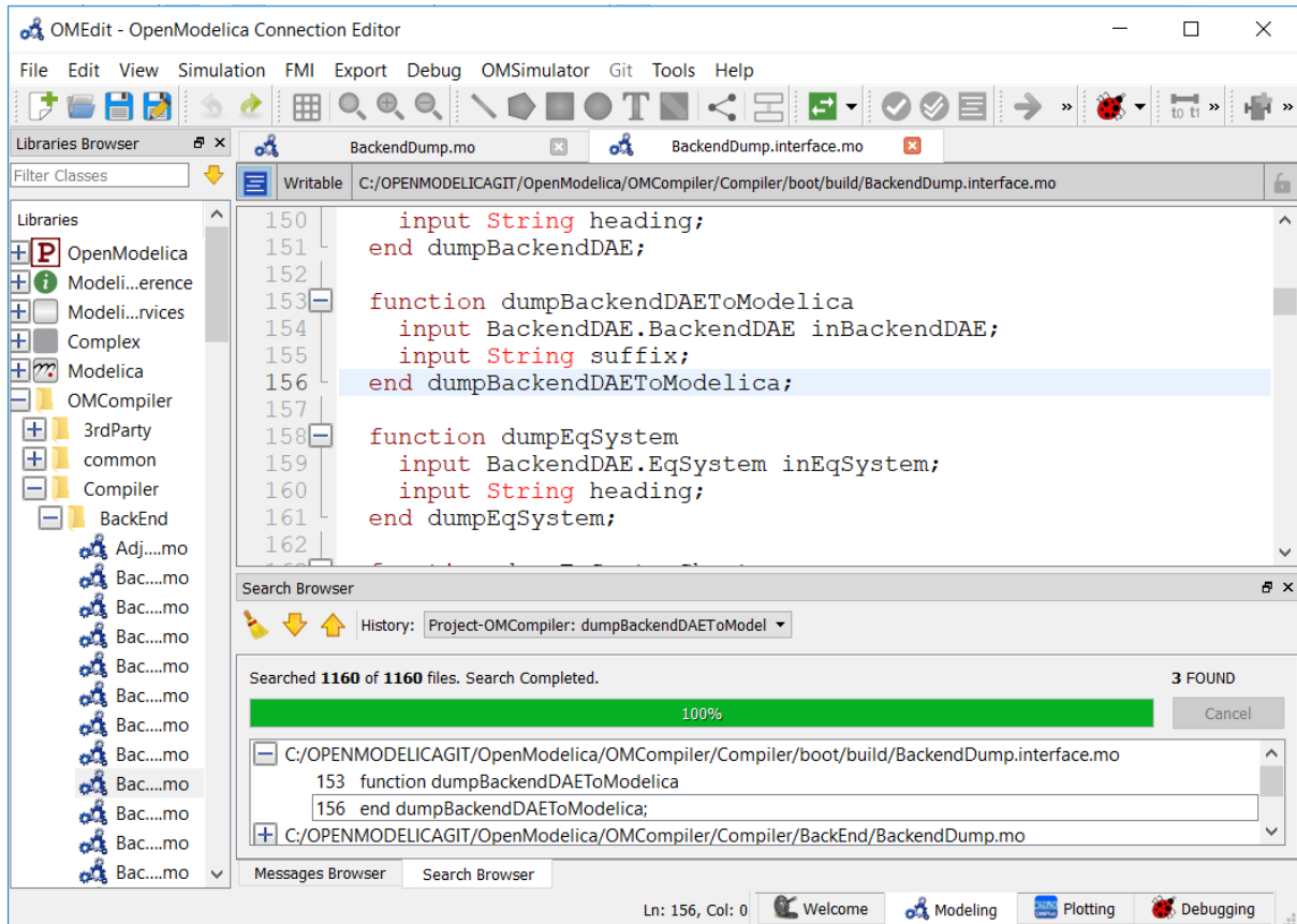
Figure 2.20: Search Results
