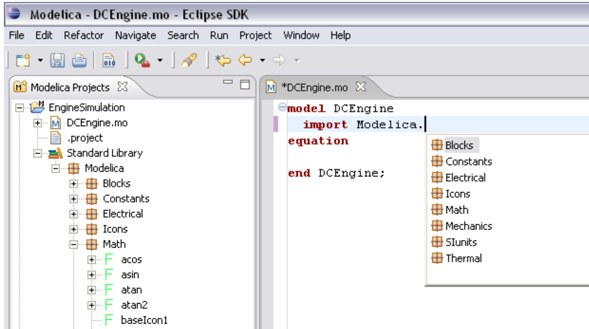
Figure 16.11: Code completion when typing a dot.
