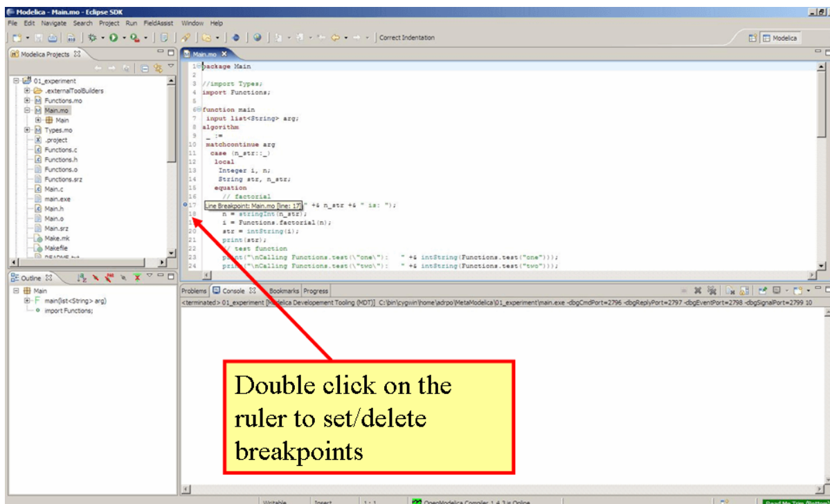
Figure 19.4: Setting/deleting breakpoints.
