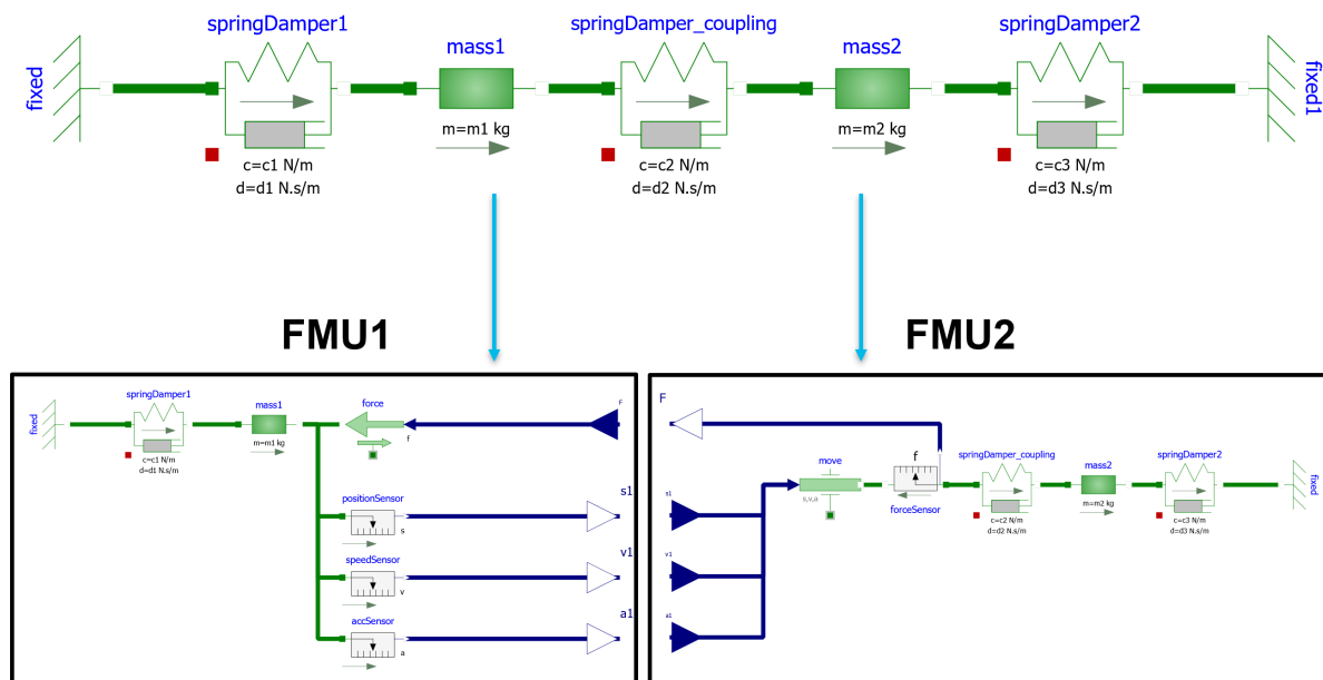
Figure 10.11: Dual mass oscillator Modelica model (diagramm view) and FMUs
