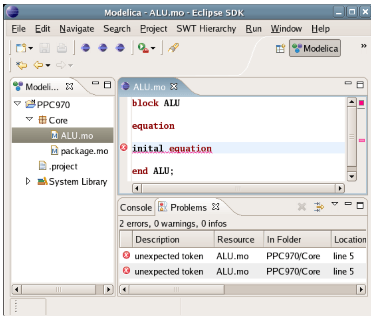
Figure 17.10: Syntax checking.
