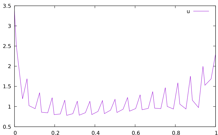
Figure 15.1: Optimization results for Batch Reactor model - input variables.
