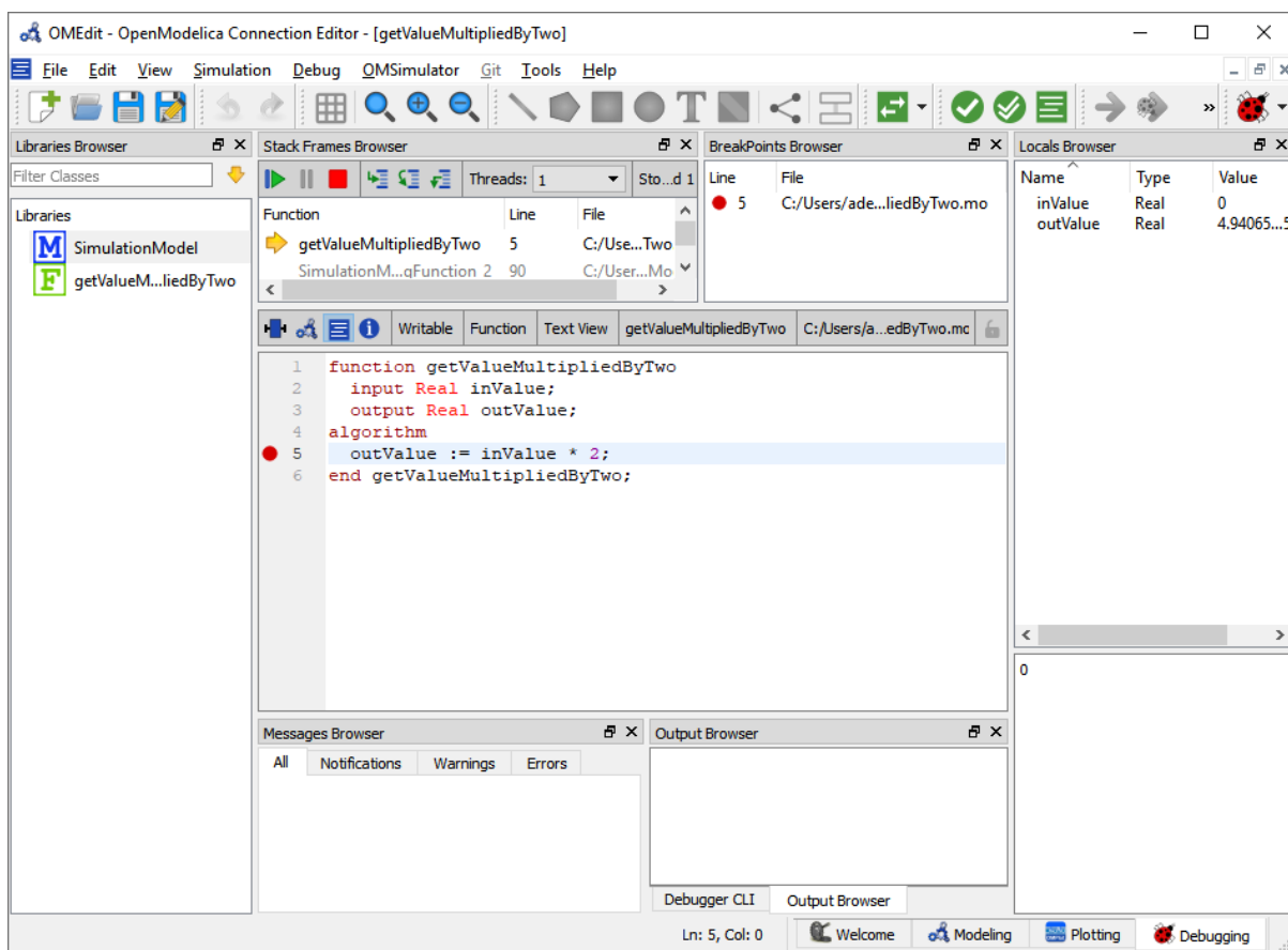
Figure 6.6: Algorithmic Debugger.
