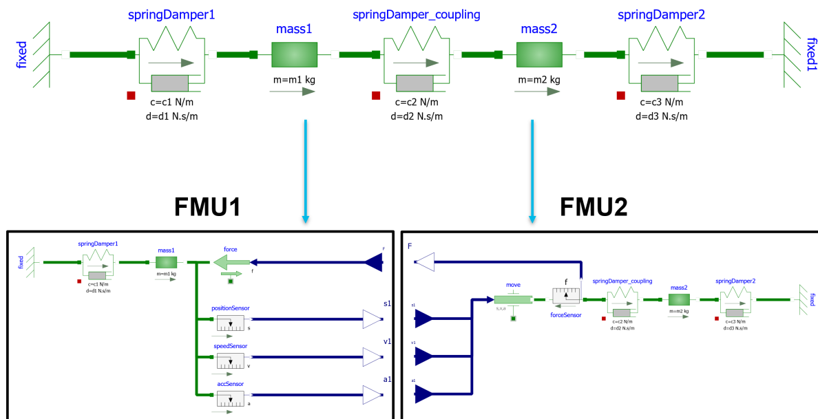
Figure 10.11: Dual mass oscillator Modelica model (diagram view) and FMUs
