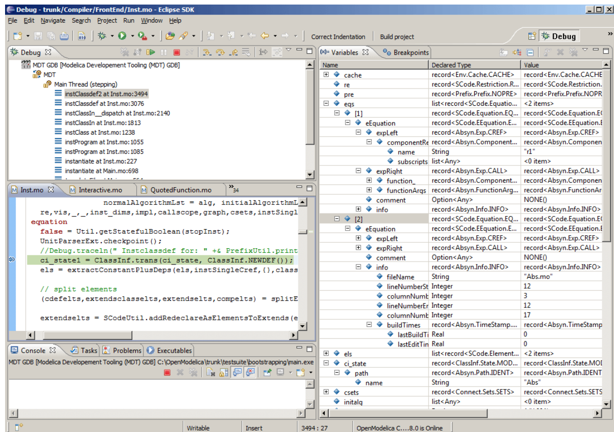
Figure 25.1: Debugging functionality.
