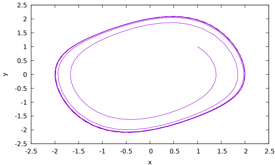
Figure 1.3: VanDerPol plotParametric(x,y)
