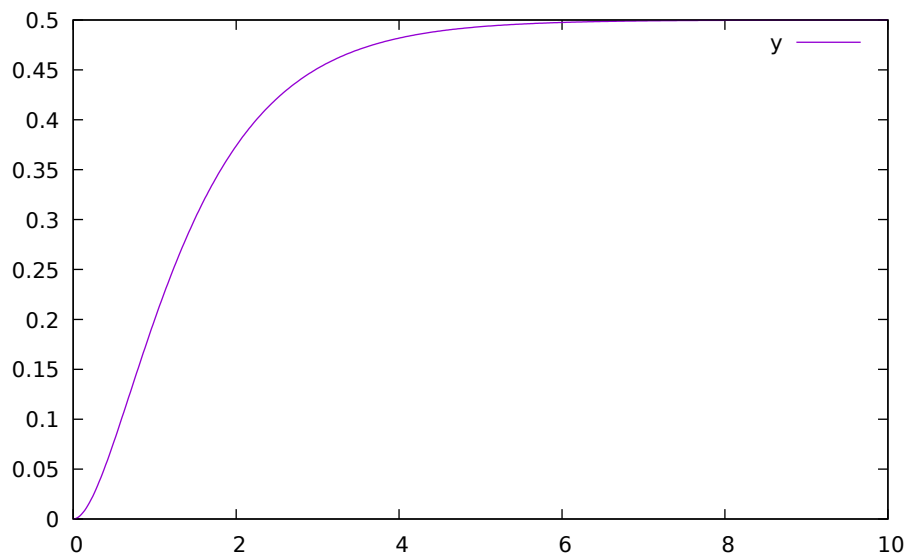
Figure 20.9: Characteristic equation with real negative roots.
