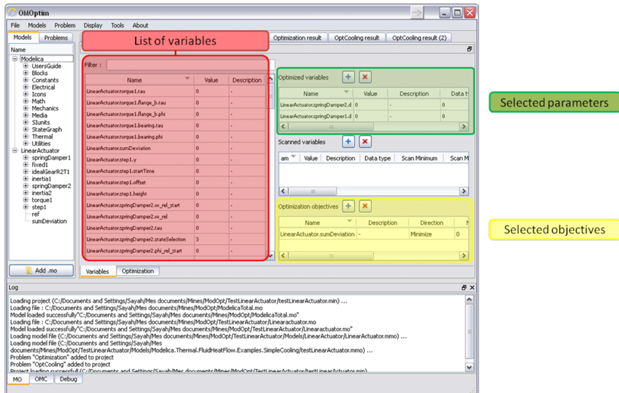
Figure 21.4: Forms for defining a new optimization problem.
