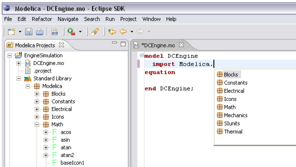
Figure 24.11: Code completion when typing a dot.
