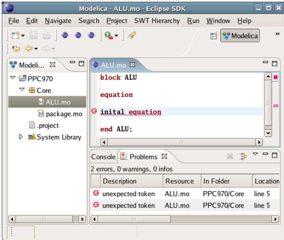
Figure 24.10: Syntax checking.
