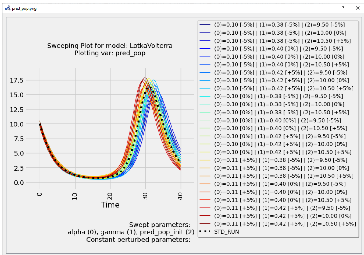
Figure 22.12: Multi-parameter sweep plot.
