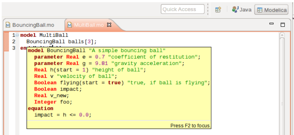
Figure 24.13: Displaying information for identifiers on hovering.
