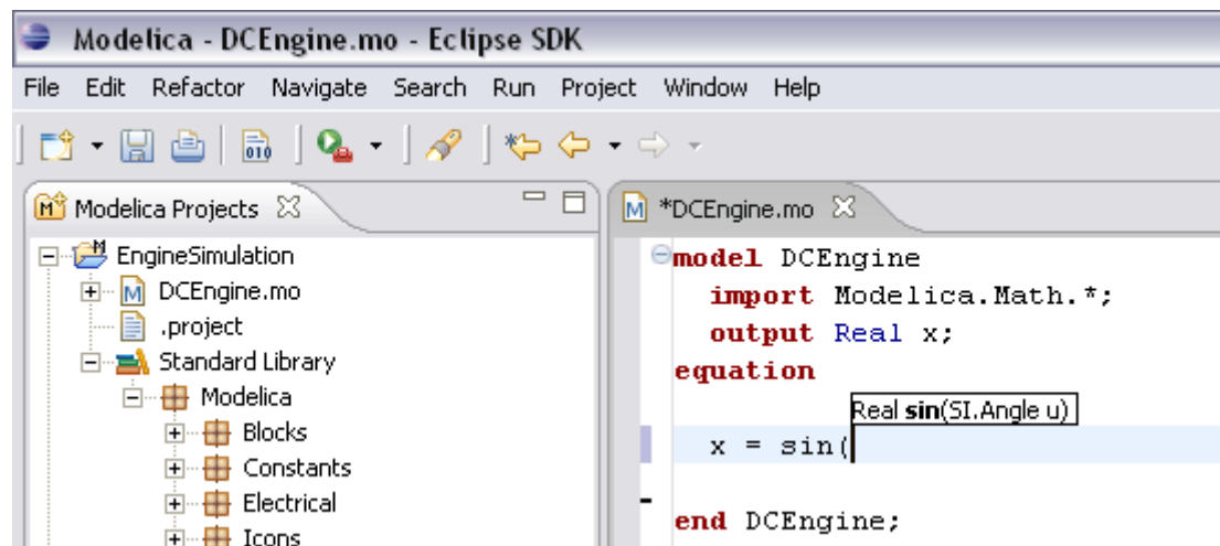
Figure 24.12: Code completion at a function call when typing left parenthesis.
