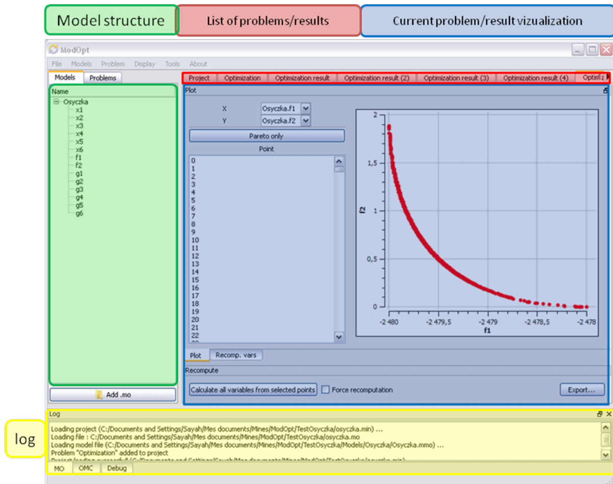
Figure 21.6: Window regions in OMOptim GUI.
