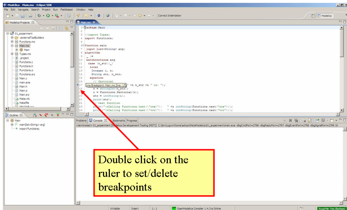
Figure 25.4: Setting/deleting breakpoints.
