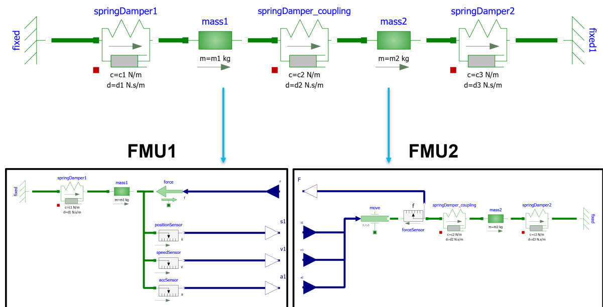
Figure 17.15: Dual mass oscillator Modelica model (diagram view) and FMUs
