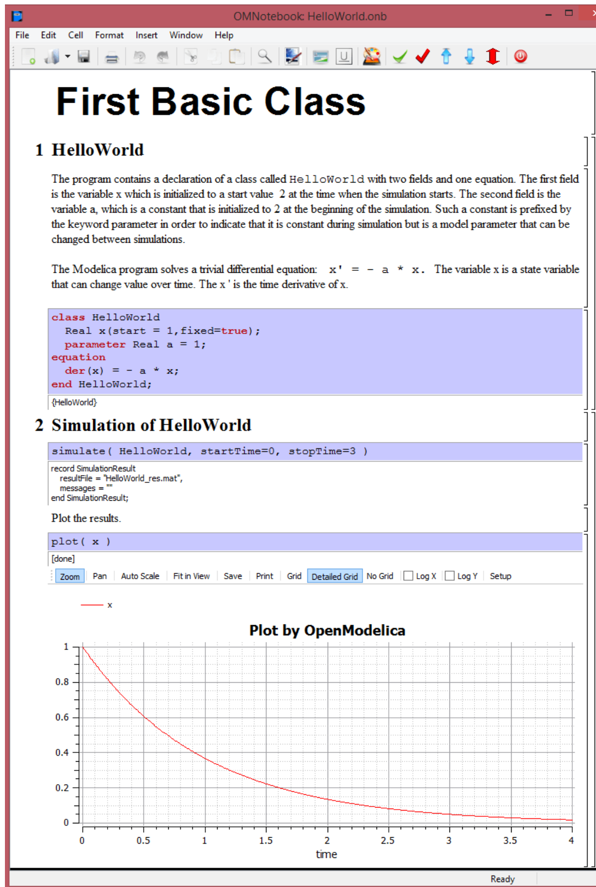
Figure 20.3: The HelloWorld class simulated and plotted using the OMNotebook version of DrModelica.
