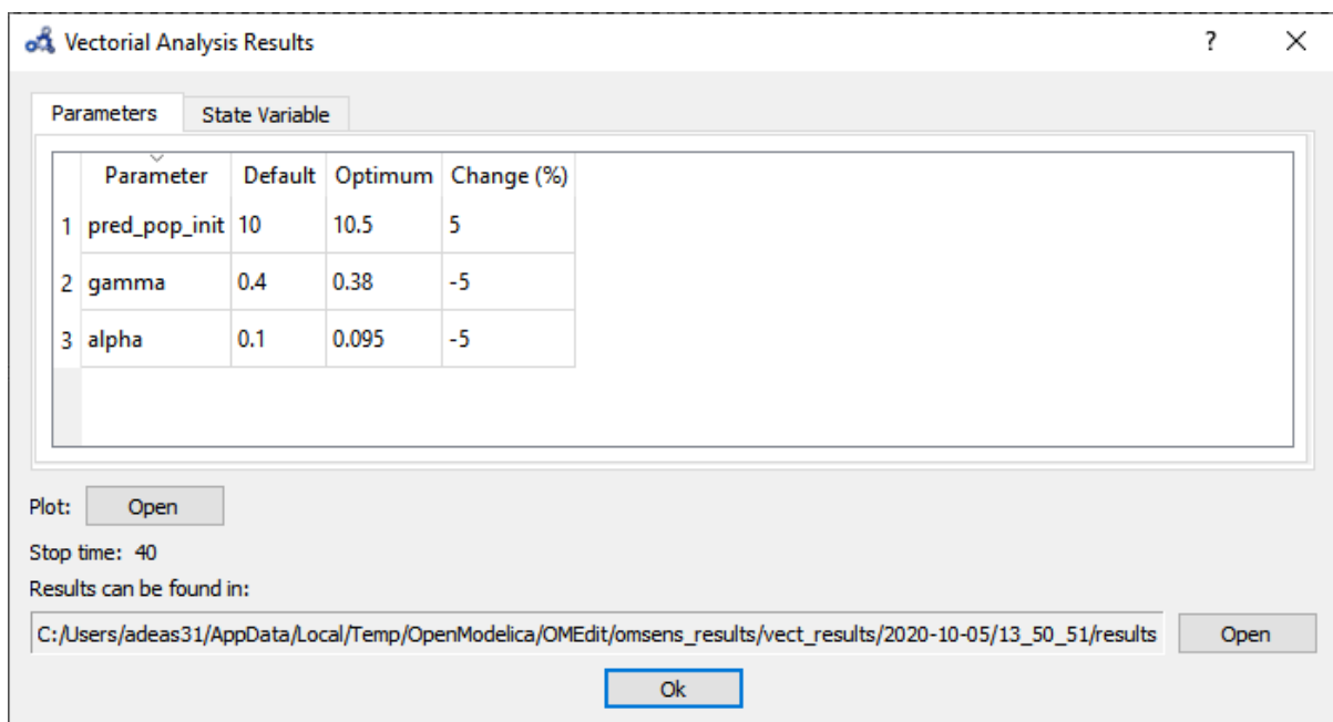
Figure 22.15: Vectorial sensitivity analysis parameters result.
