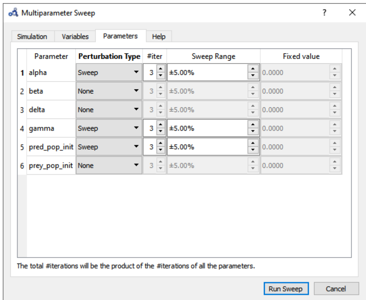
Figure 22.10: Multi-parameter sweep parameters.
