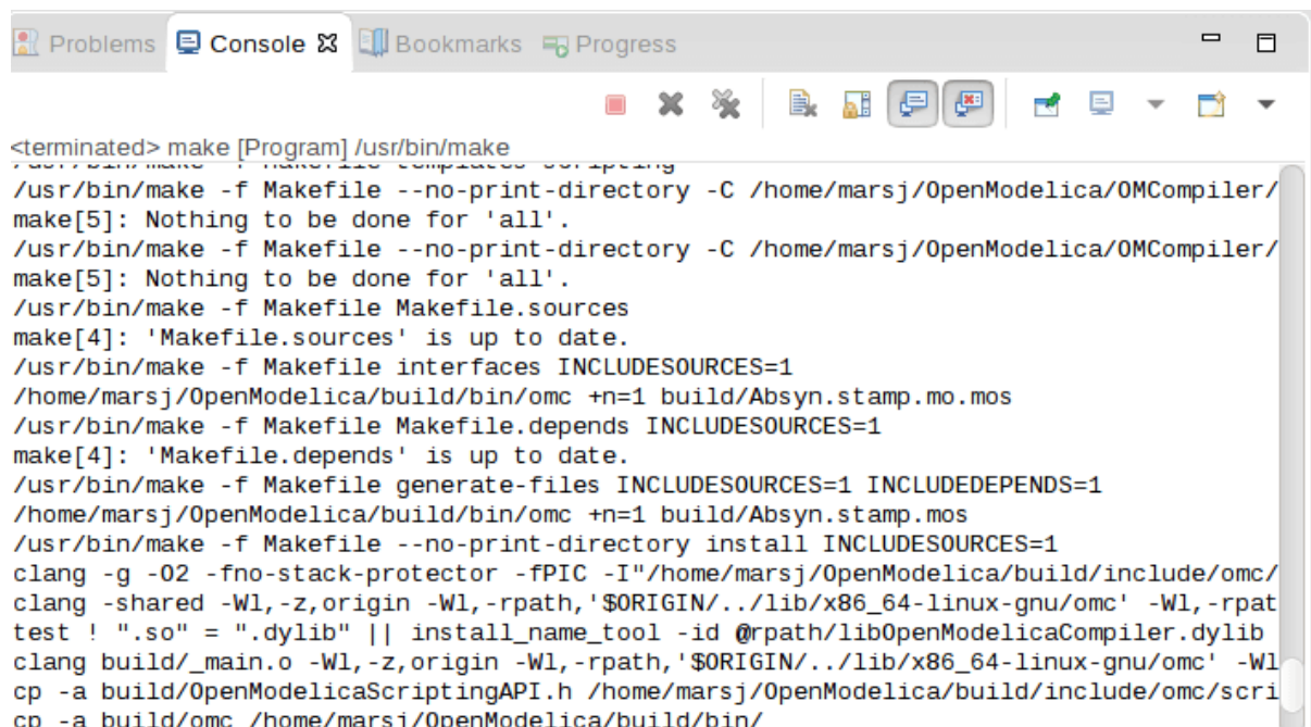
Figure 24.6: Eclipse - building a project, resulting log.
