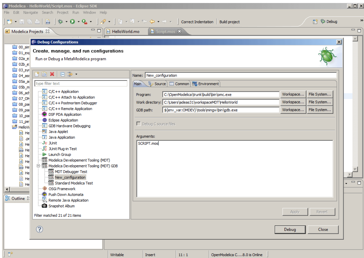
Figure 25.3: Creating the Debug Configuration.
