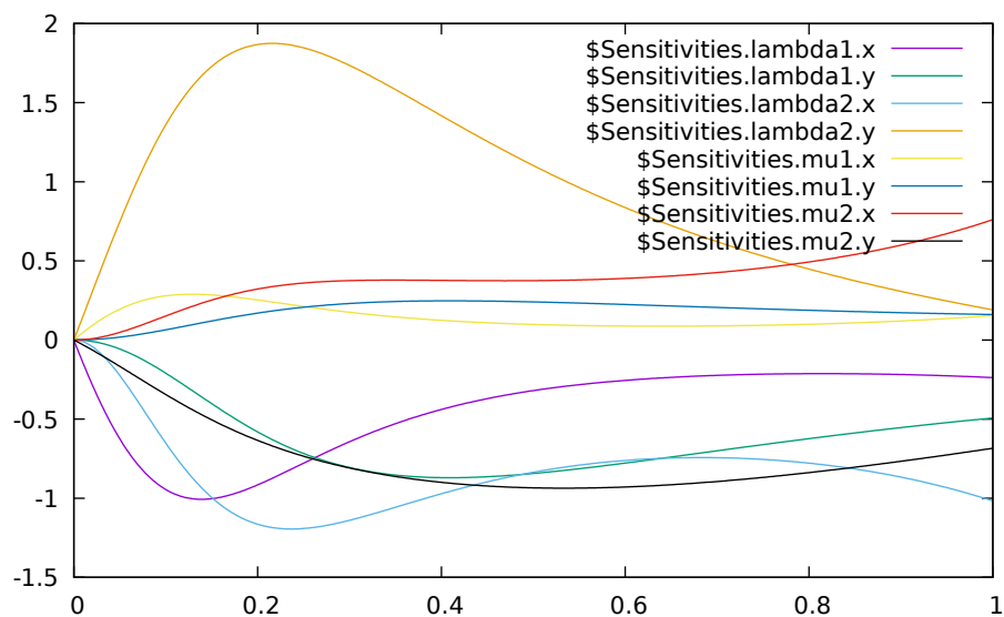
Figure 22.1: Results of the sensitivities calculated by IDA solver.
