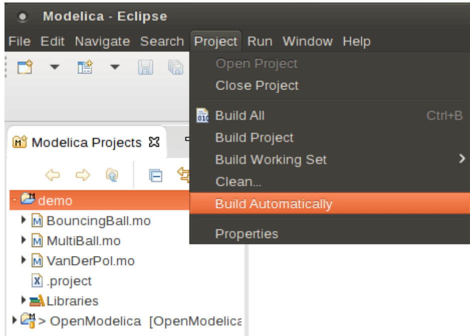
Figure 24.3: Eclipse Setup - disable automatic build for the projects.
