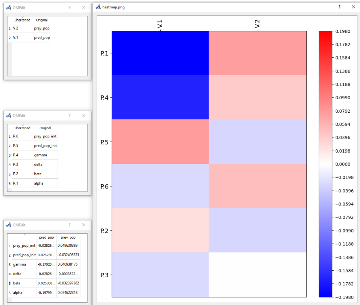
Figure 22.9: Individual sensitivity analysis heatmap.
