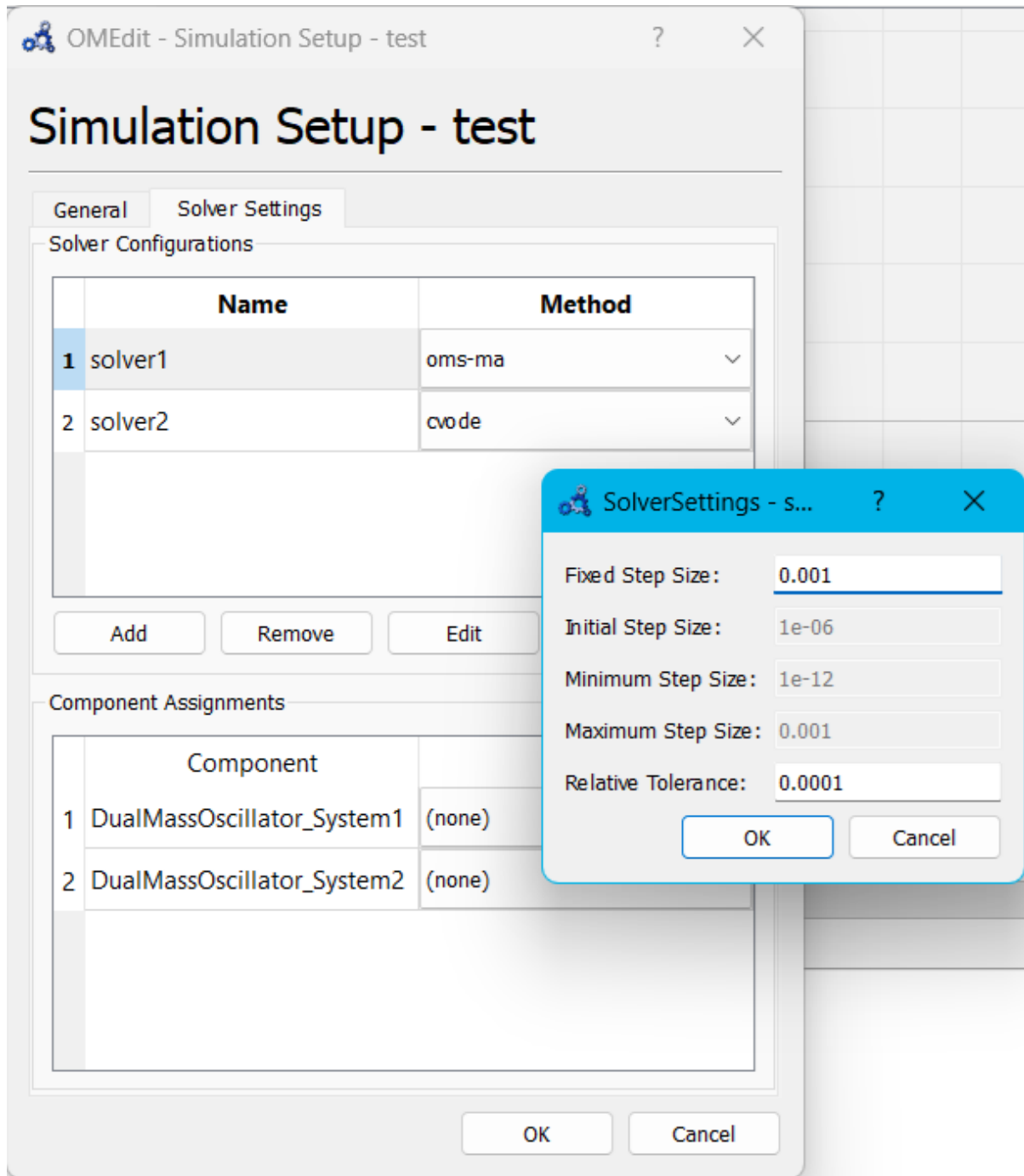
Figure 17.13: OMEdit: Solver Settings dialog.
