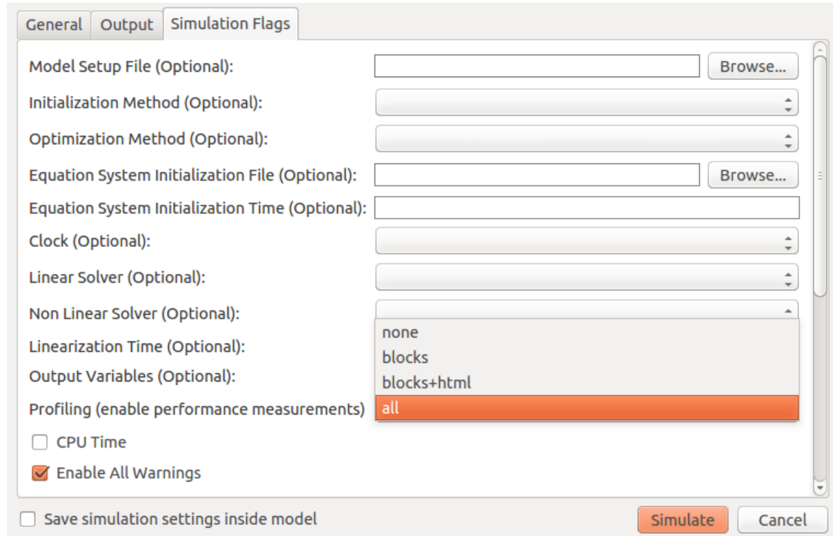
Figure 26.1: Setting up the profiler from OMEdit.
