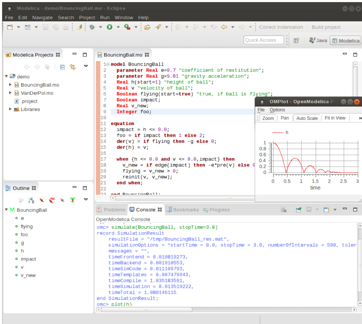
Figure 24.16: Simulation from MDT Console.
