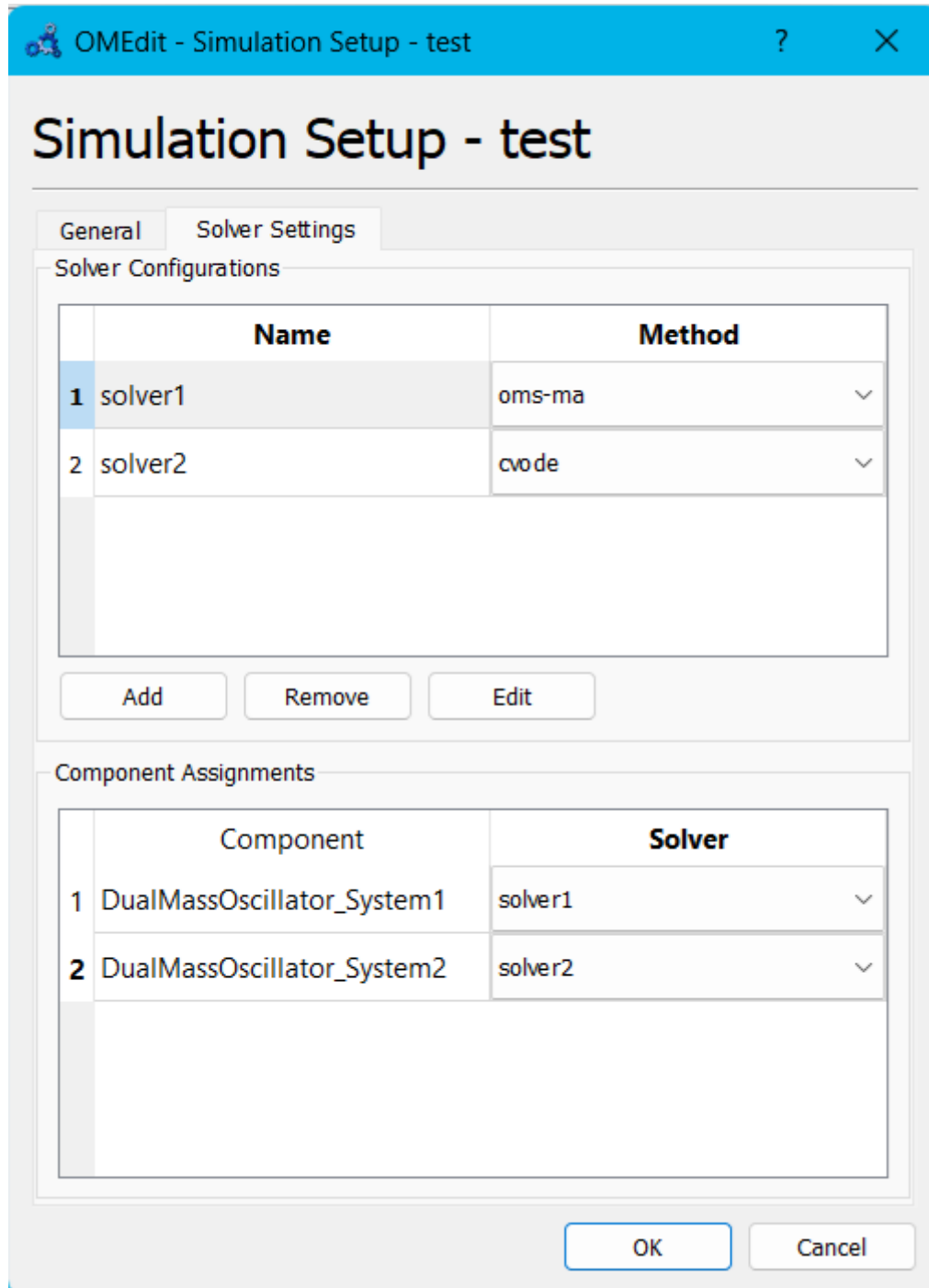
Figure 17.14: OMEdit: Solver Assignments in Components
