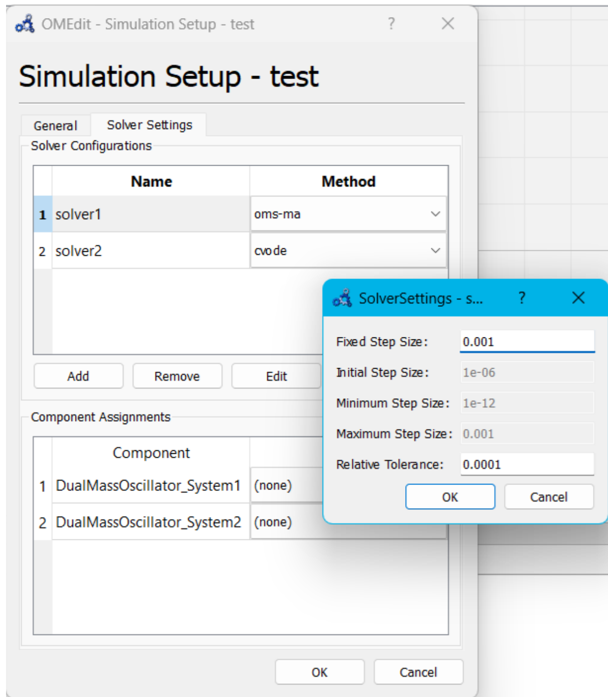
Figure 14.14: OMEdit: Solver Settings dialog.
