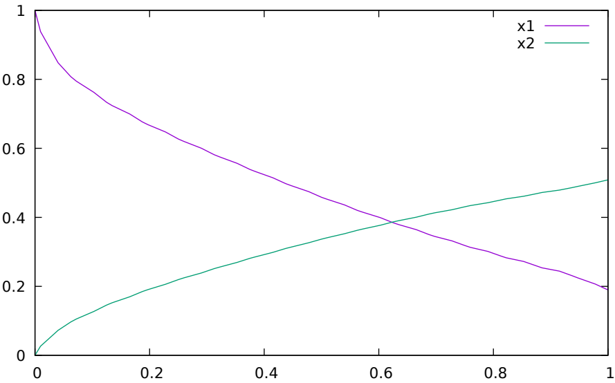
Figure 18.2: Optimization results for Batch Reactor model - state variables.
