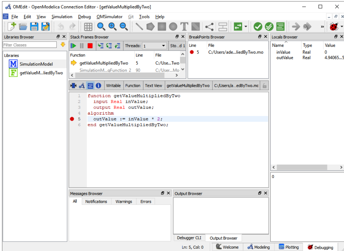
Figure 8.6: Algorithmic Debugger.
