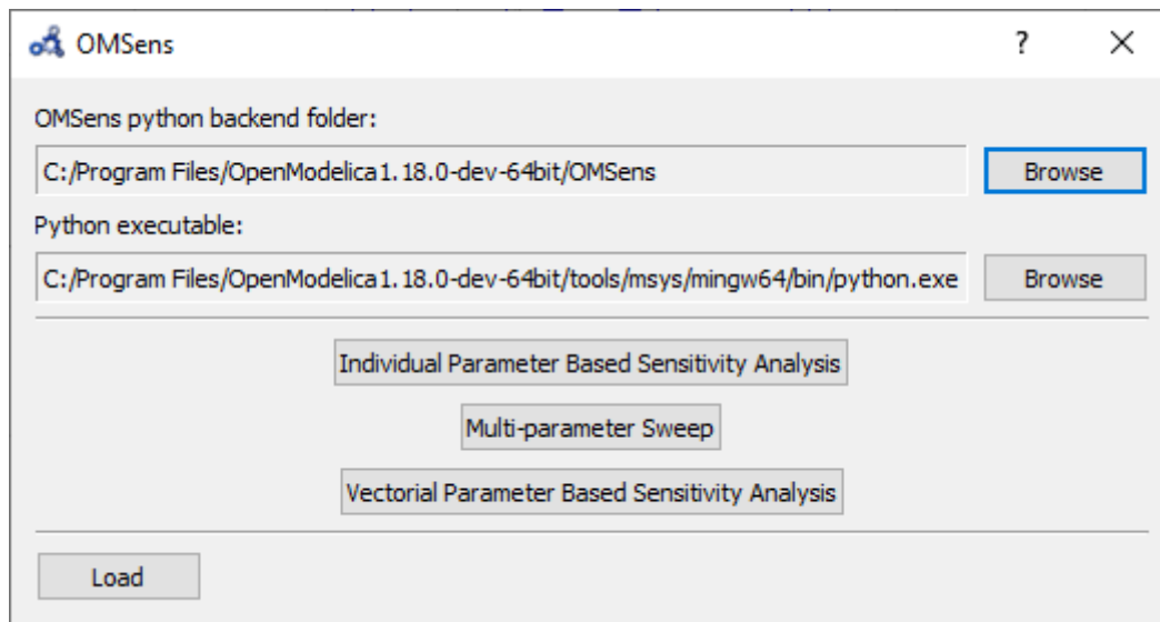
Figure 19.3: OMSens window.
