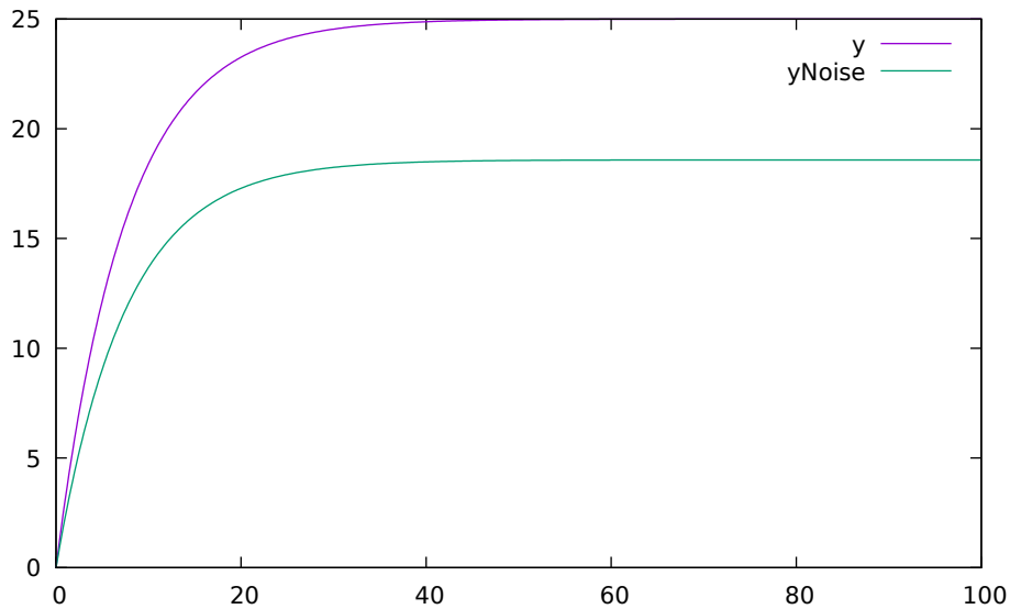
Figure 17.8: Open loop control example.
