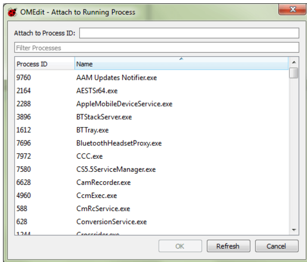
Figure 8.5: Attach to Running Process.
