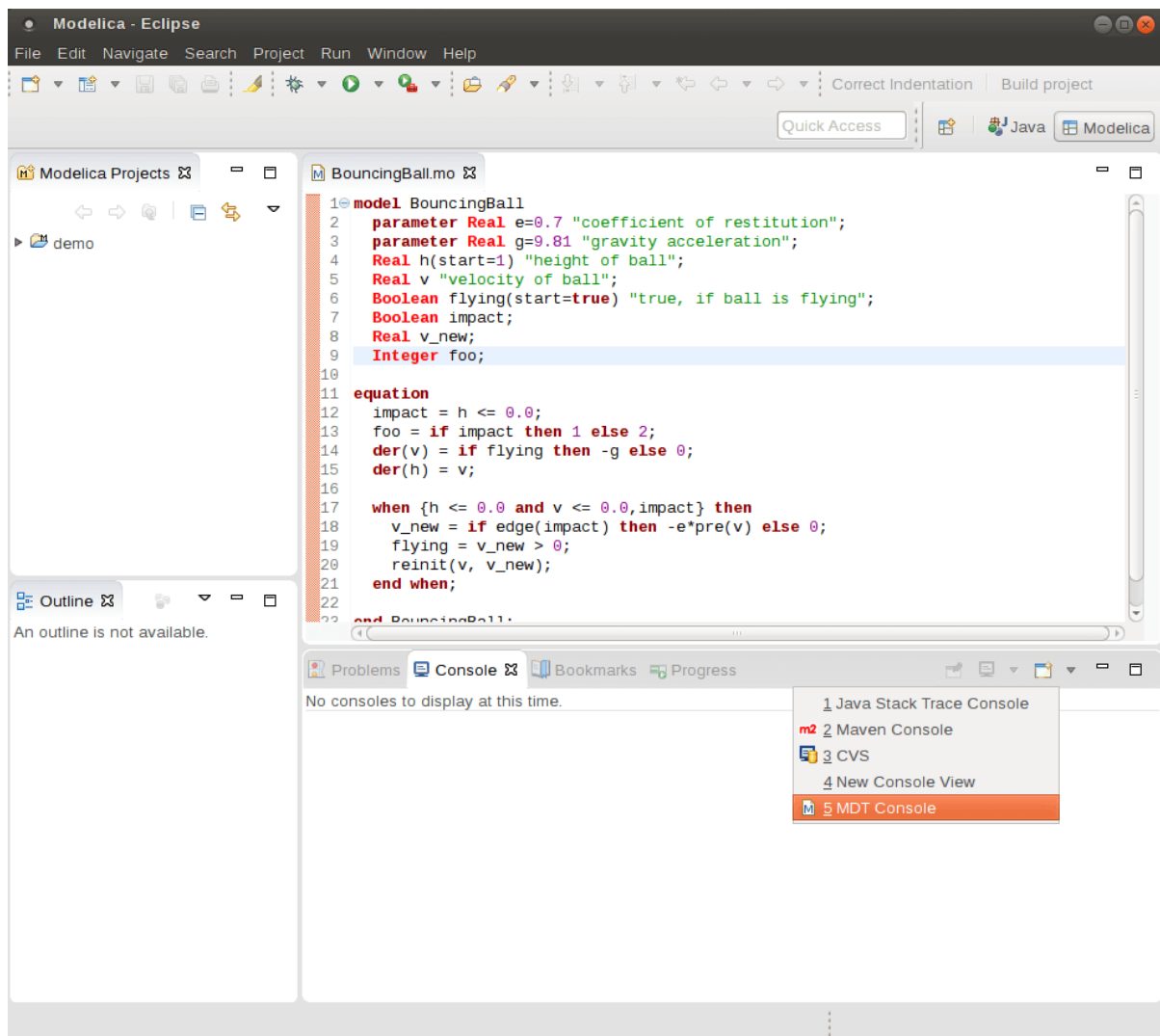
Figure 21.15: Activate the MDT Console.
