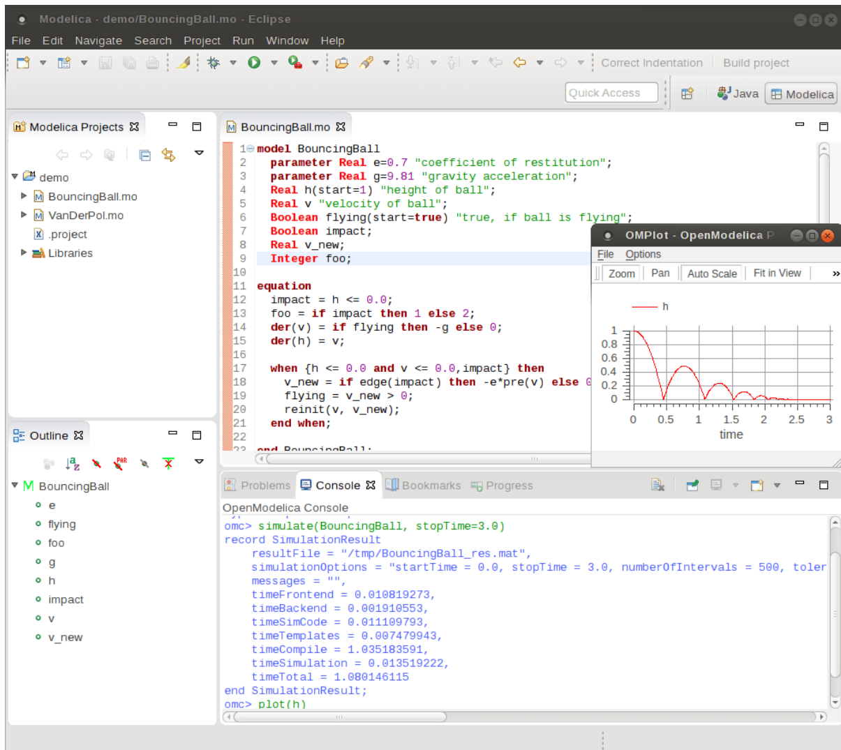
Figure 21.16: Simulation from MDT Console.
