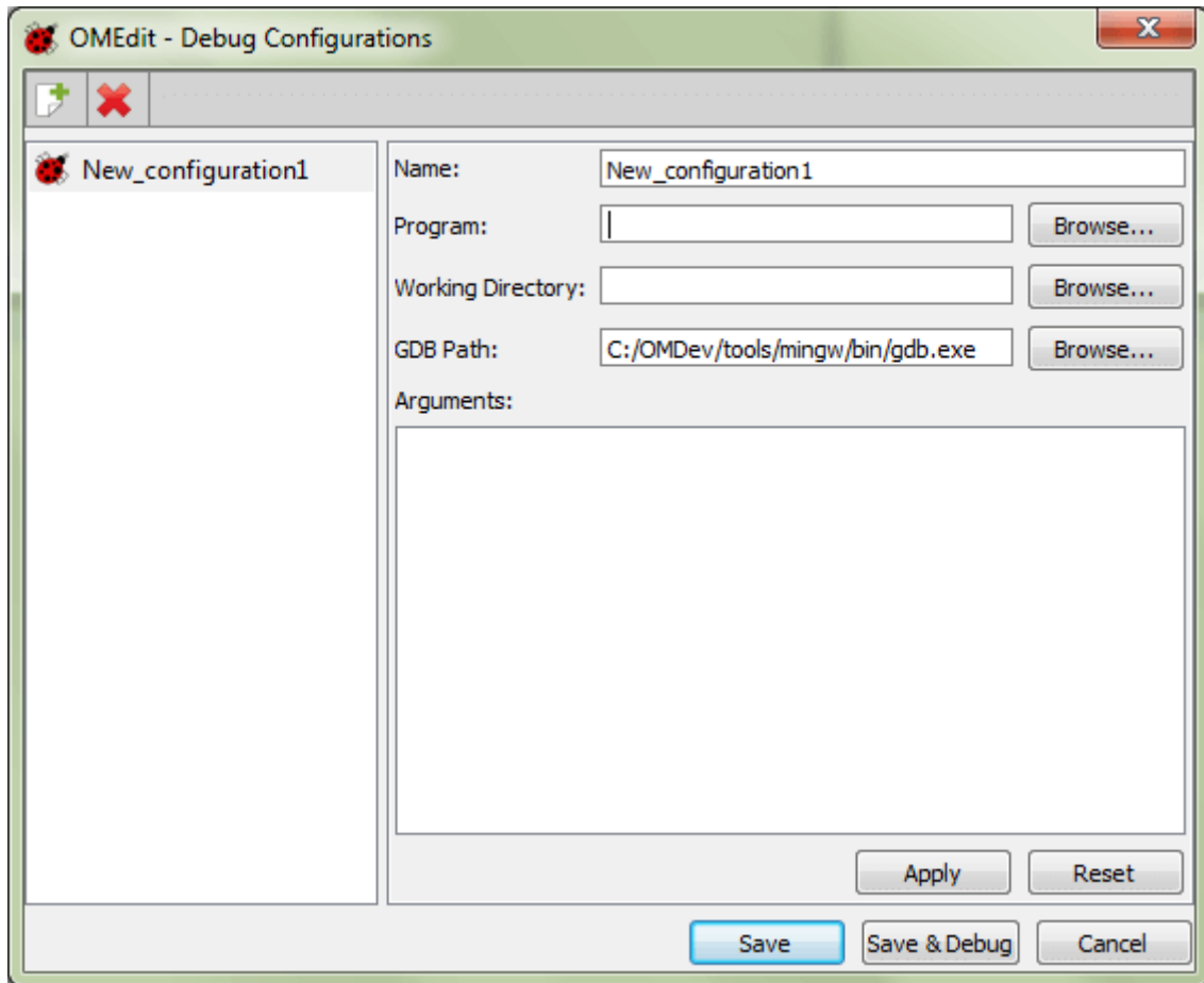
Figure 8.4: Debug Configurations.
