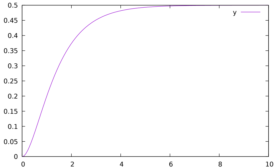
Figure 17.11: Characteristic equation with real negative roots.
