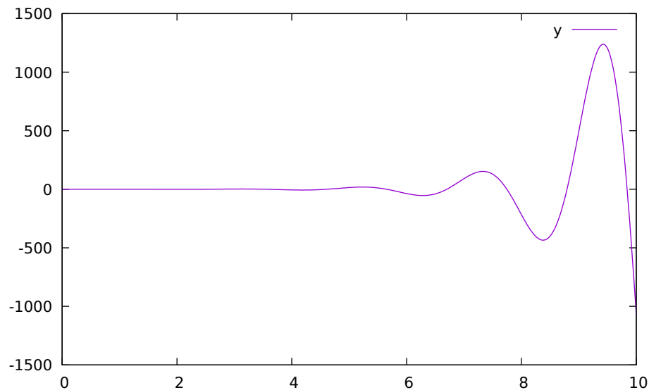
Figure 17.12: Characteristic equation with imaginary roots with positive real part.
