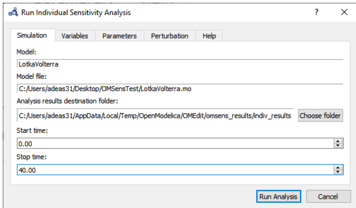
Figure 19.4: Run individual sensitivity analysis.
