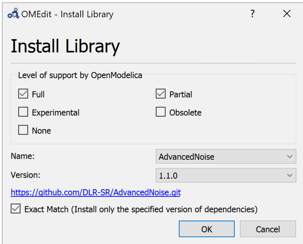
Figure 3.13: Install Library.
