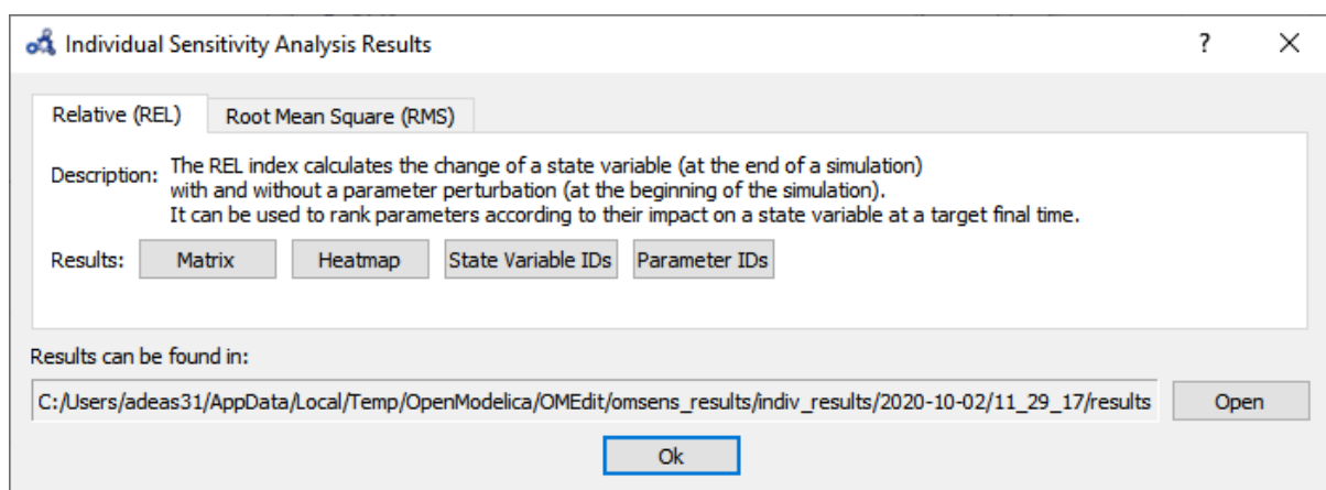
Figure 19.8: Individual sensitivity analysis results.
