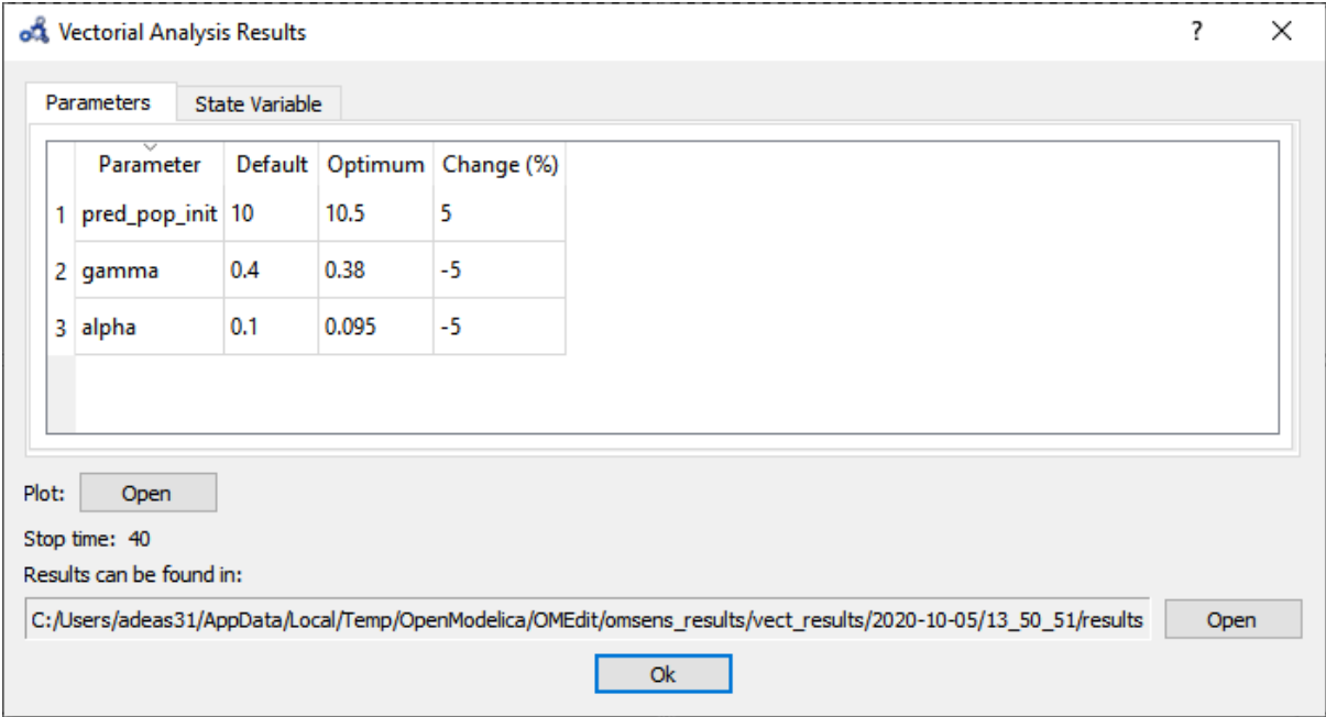
Figure 19.15: Vectorial sensitivity analysis parameters result.
