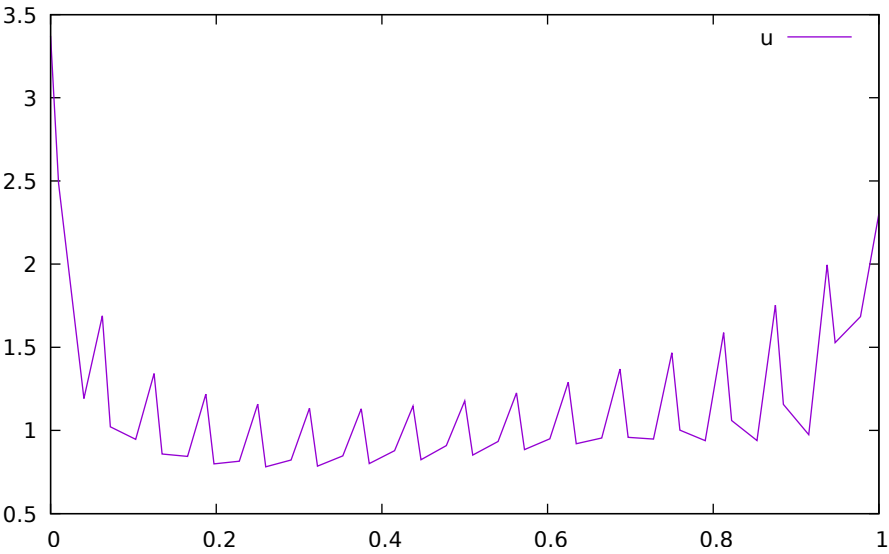
Figure 18.1: Optimization results for Batch Reactor model - input variables.
