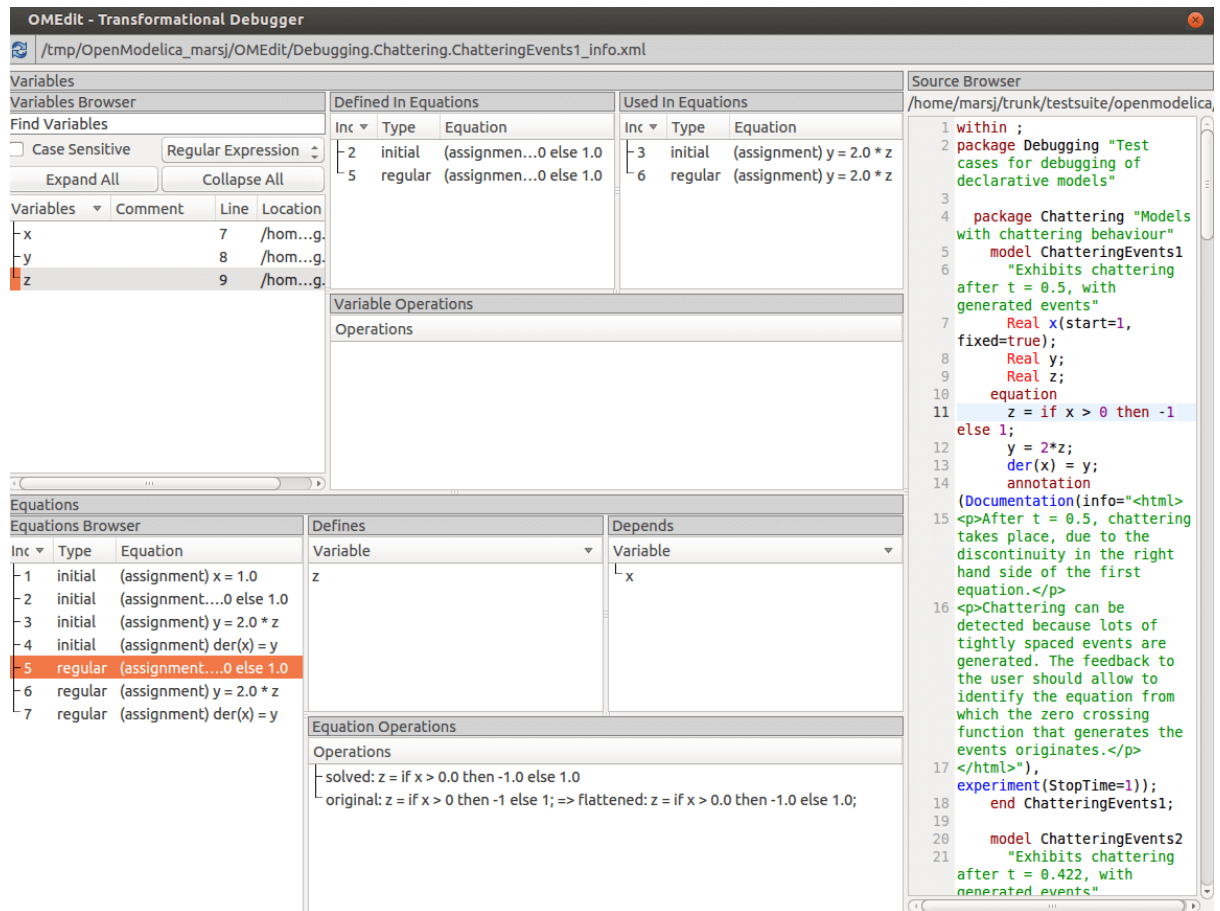
Figure 8.2: Transformations Browser.
