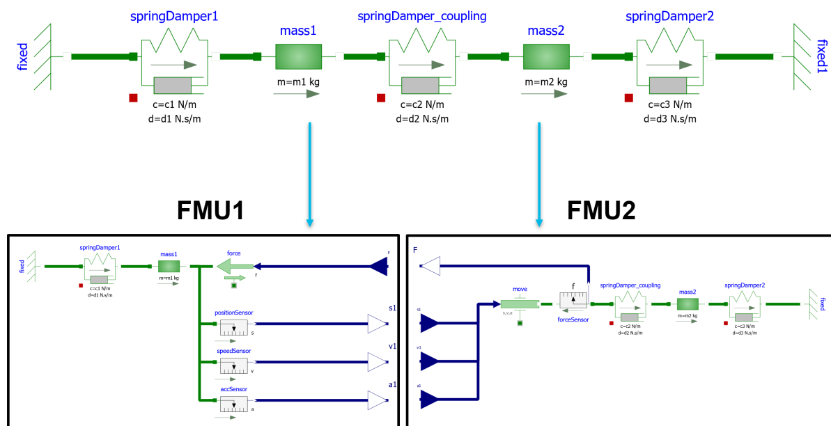
Figure 14.16: Dual mass oscillator Modelica model (diagram view) and FMUs
