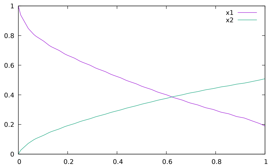
Figure 18.2: Optimization results for Batch Reactor model - state variables.
