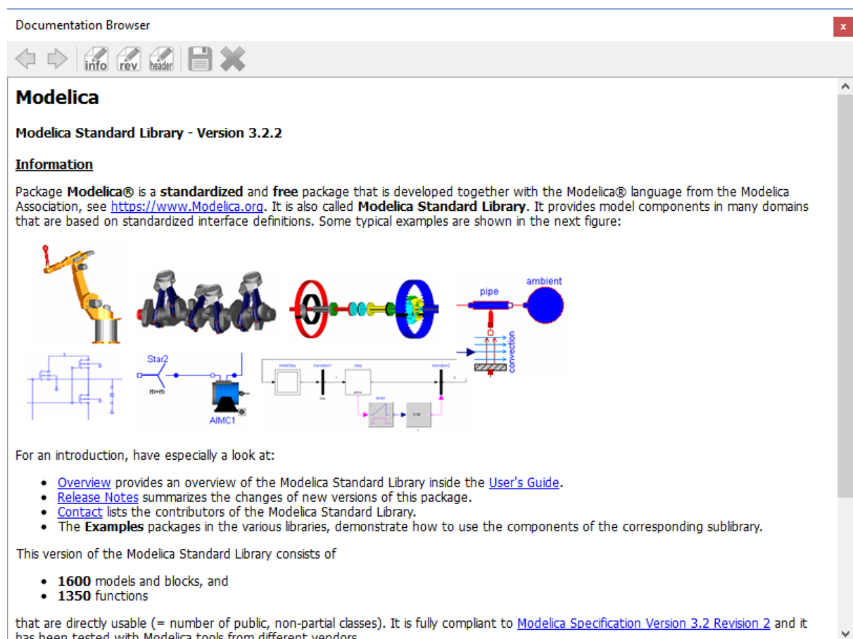
Figure 3.3: Documentation Browser.
