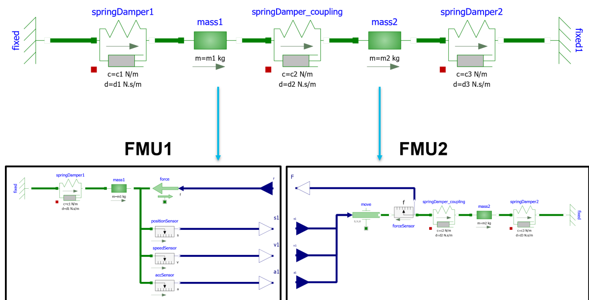
Figure 14.11: Dual mass oscillator Modelica model (diagram view) and FMUs
