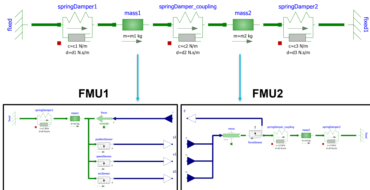
Figure 14.11: Dual mass oscillator Modelica model (diagramm view) and FMUs
