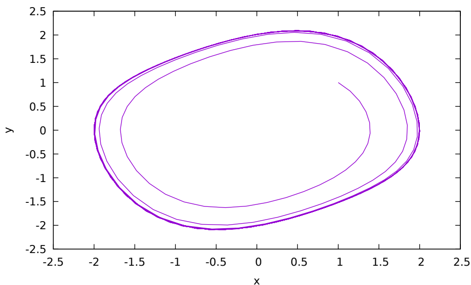
Figure 1.4: VanDerPol plotParametric(x,y)
