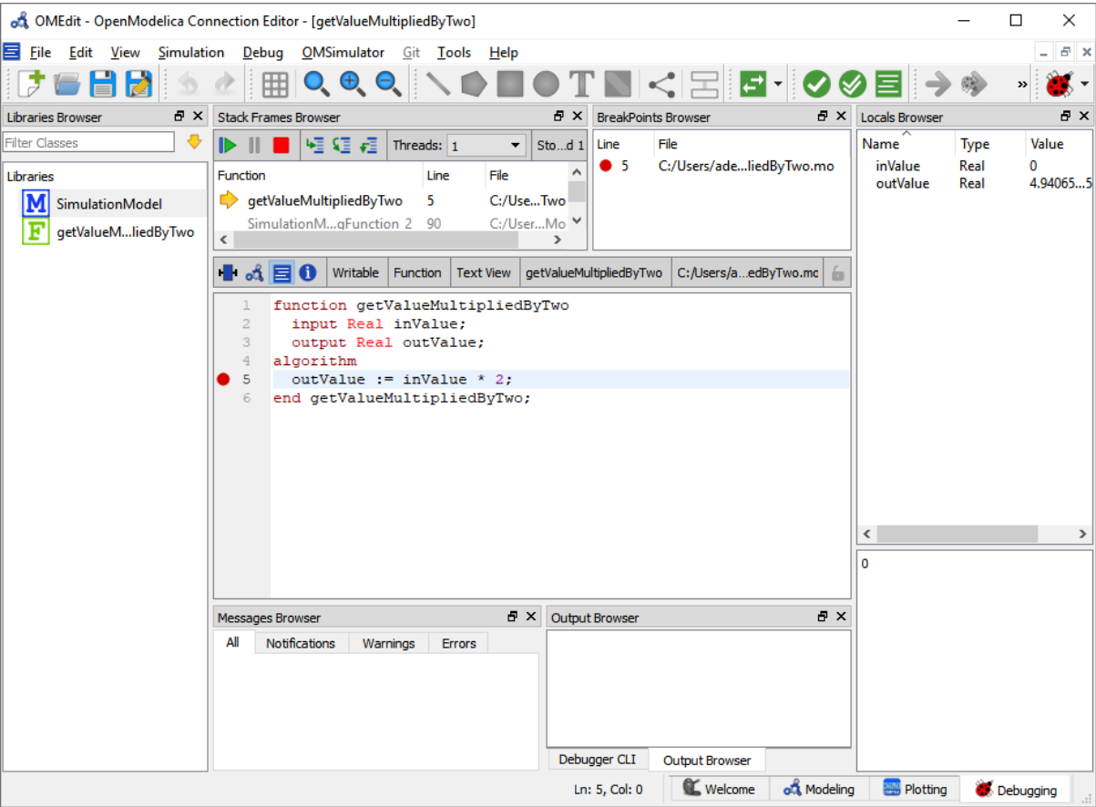
Figure 7.6: Algorithmic Debugger.
