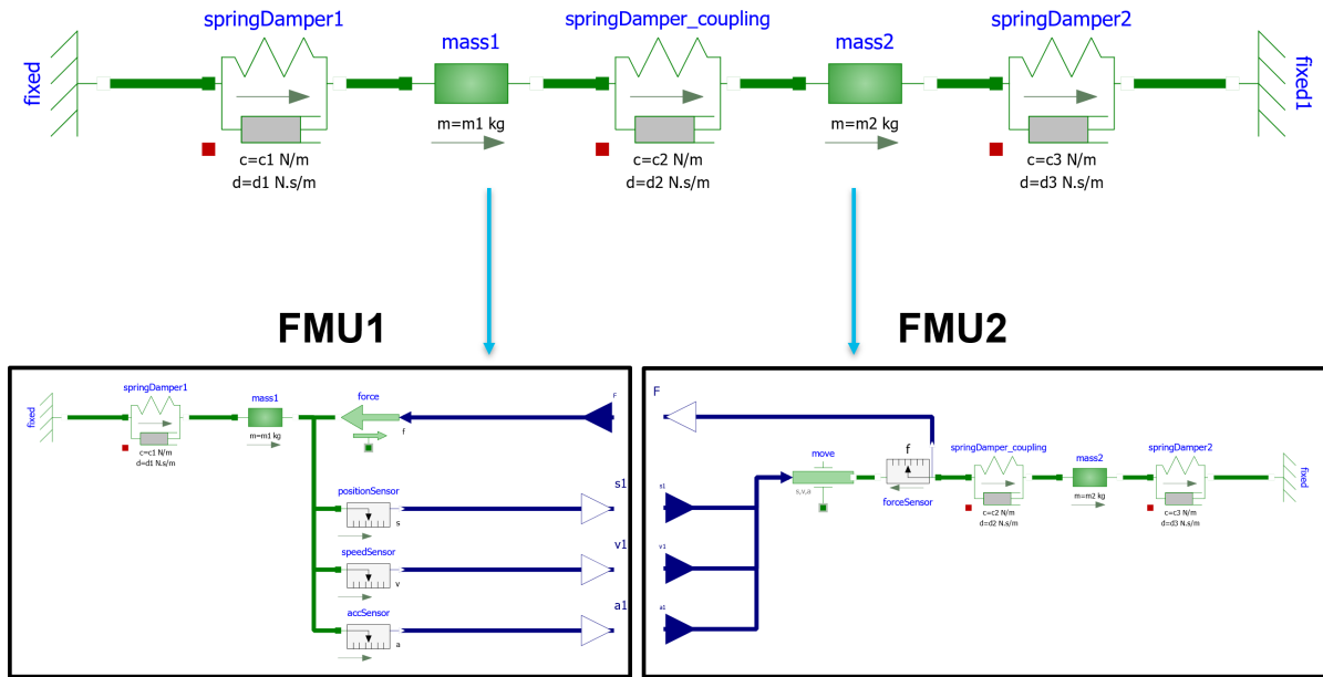
Figure 13.11: Dual mass oscillator Modelica model (diagram view) and FMUs
