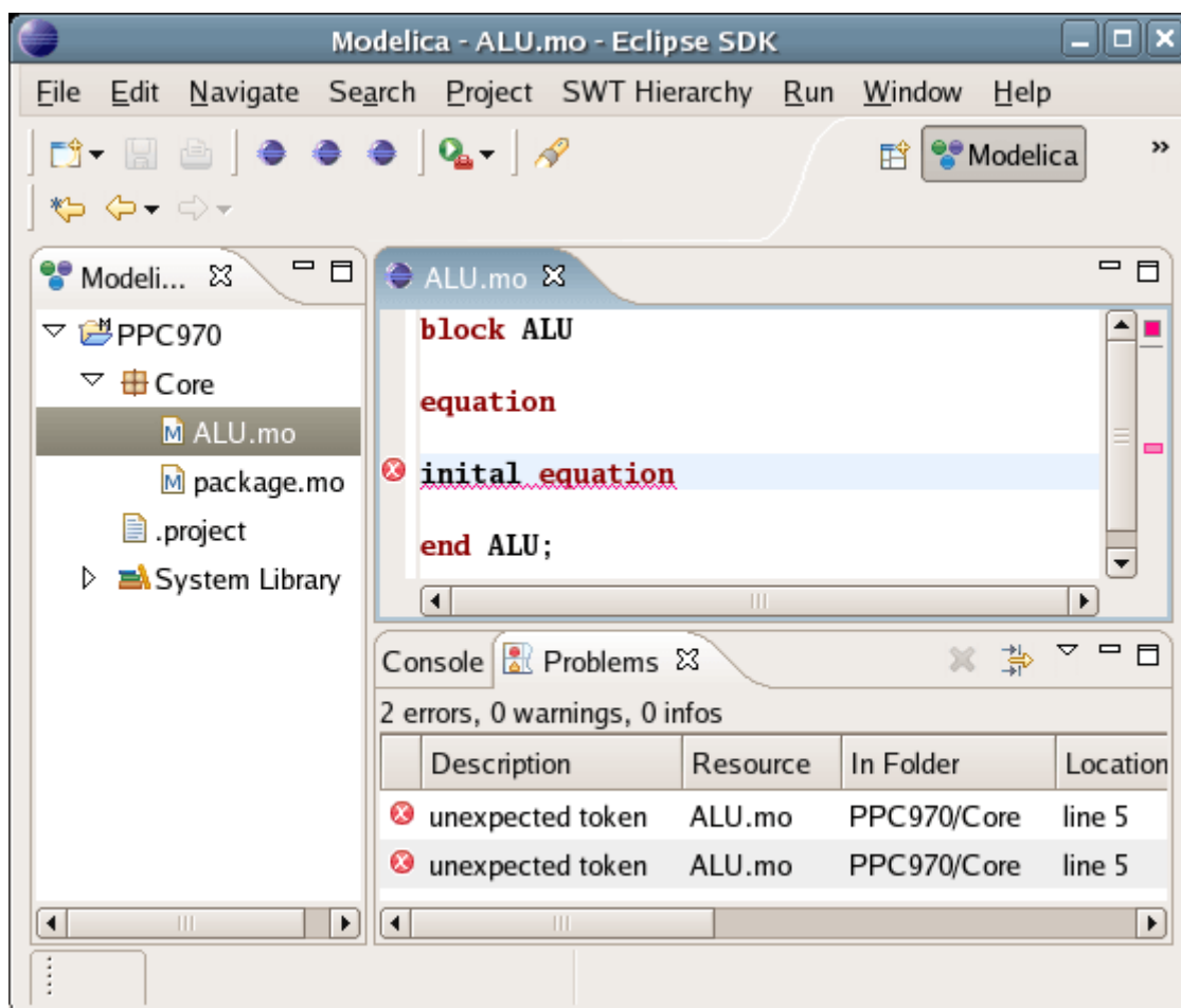
Figure 20.10: Syntax checking.
