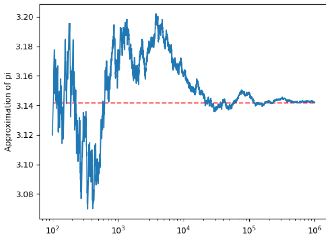
Figure 13.1: Results of the above batch simulation which approximates the value of pi
