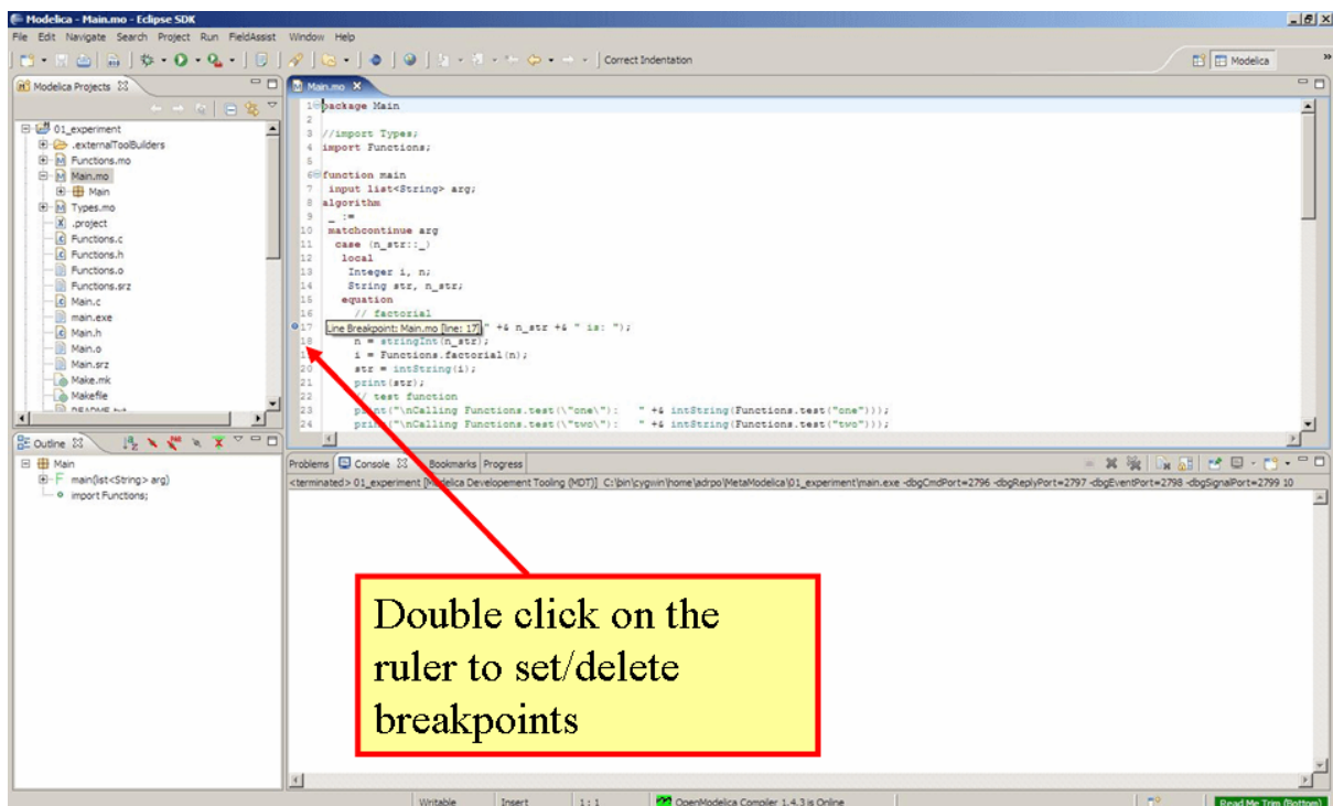
Figure 20.4: Setting/deleting breakpoints.
