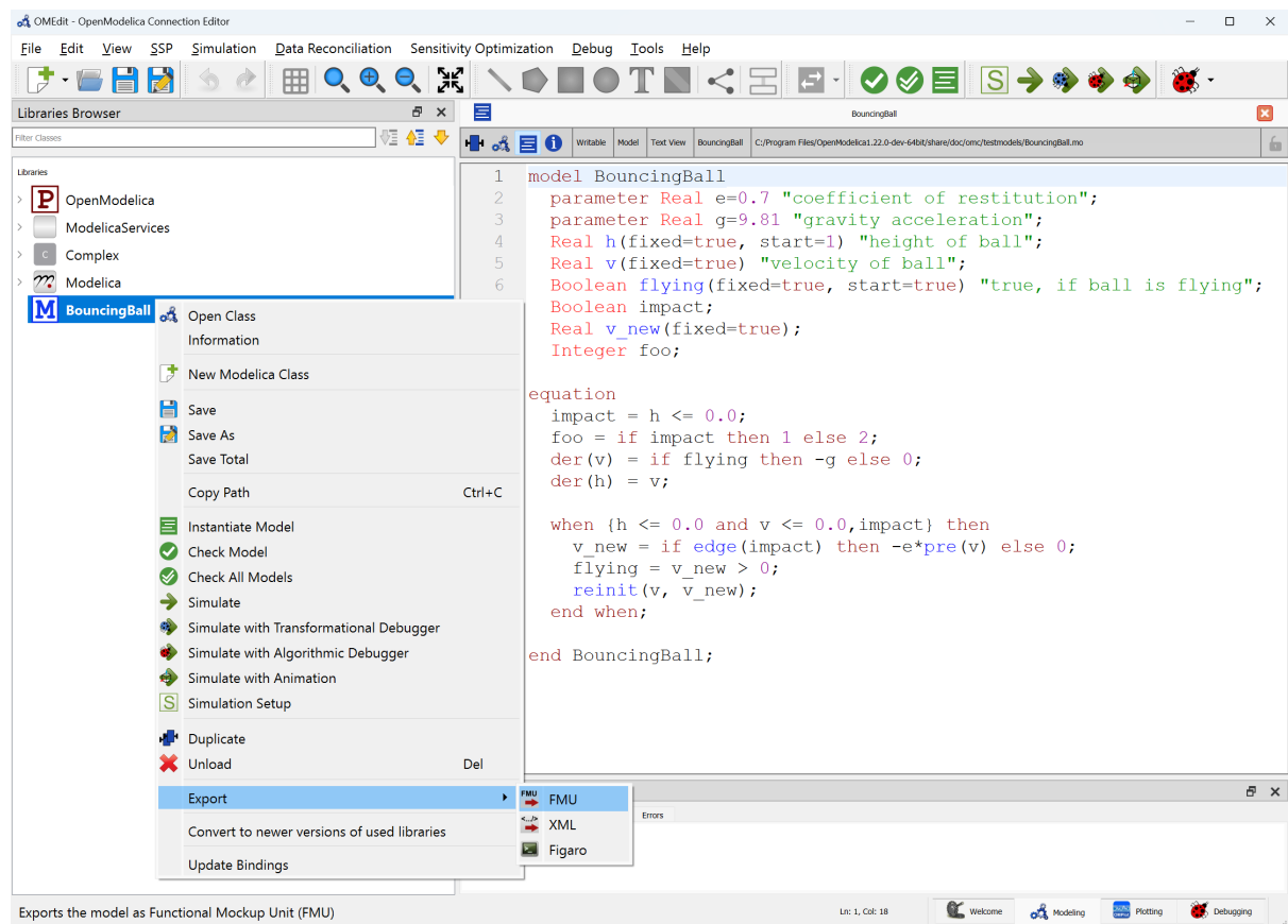
Figure 10.1: FMI Export.
