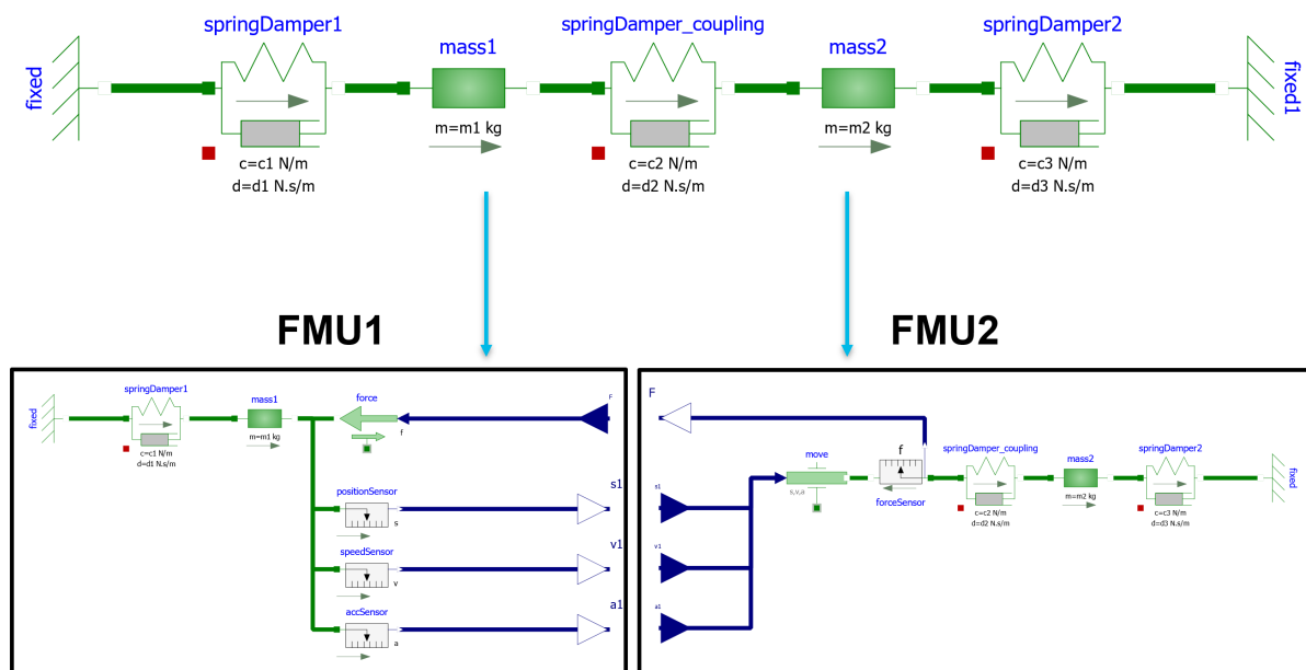
Figure 11.11: Dual mass oscillator Modelica model (diagram view) and FMUs
