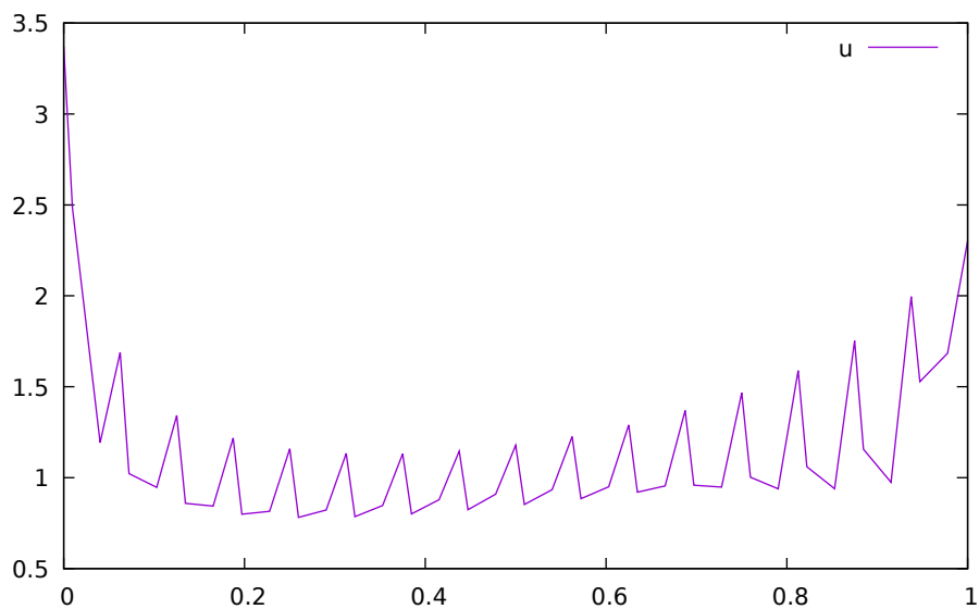
Figure 14.1: Optimization results for Batch Reactor model – input variables.
