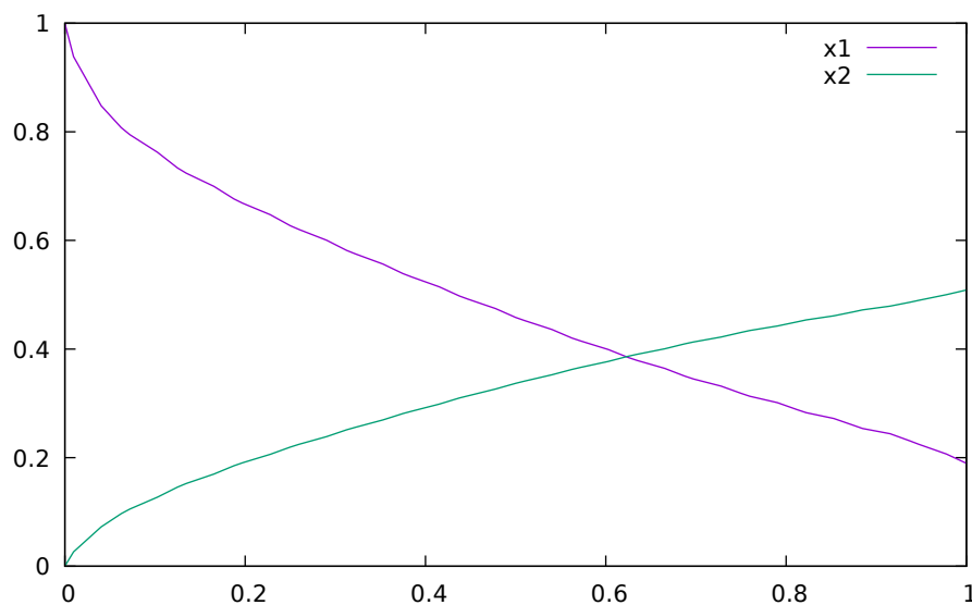
Figure 16.2: Optimization results for Batch Reactor model - state variables.
