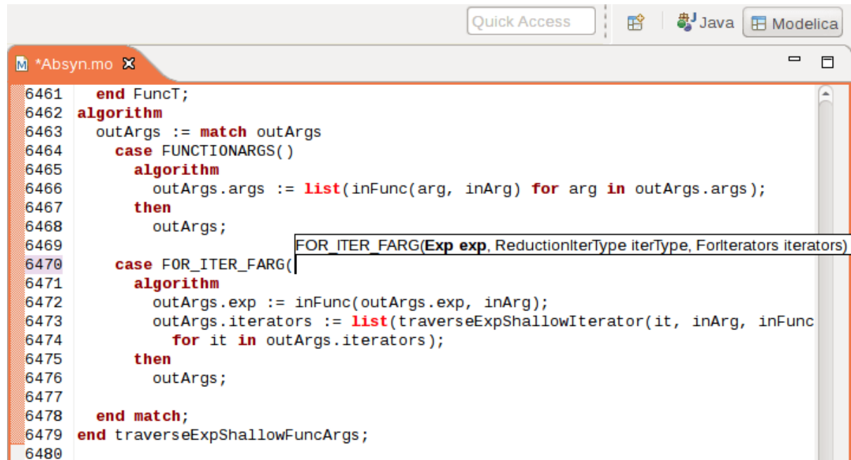
Figure 15.14: Code assistance when writing cases with records in MetaModelica.
