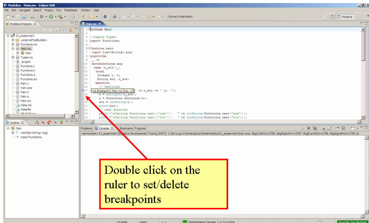
Figure 16.4: Setting/deleting breakpoints.
