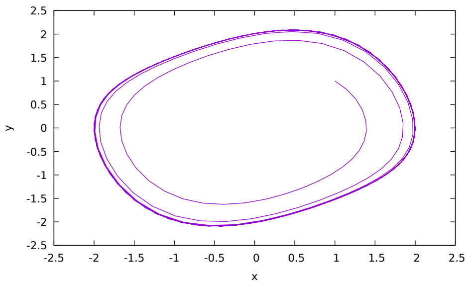
Figure 1.3: VanDerPol plotParametric(x,y)
