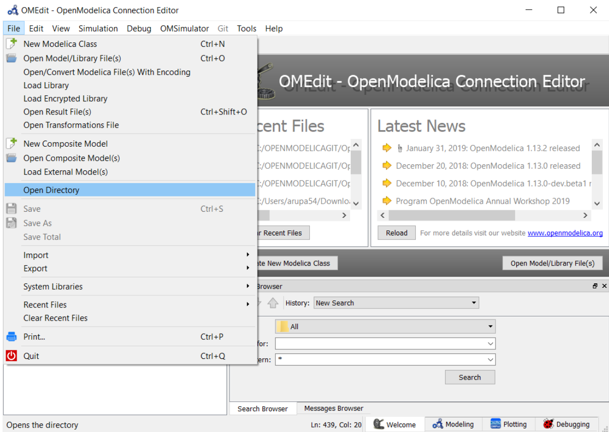
Figure 2.17: open-directory
