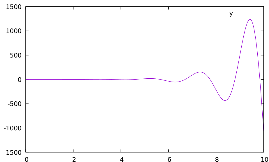
Figure 11.10: Characteristic equation with imaginary roots with positive real part.
