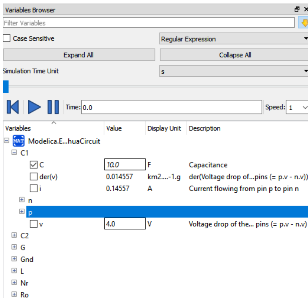
Figure 2.4: Variables Browser.
