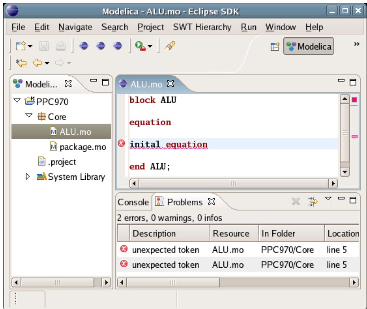
Figure 15.10: Syntax checking.
