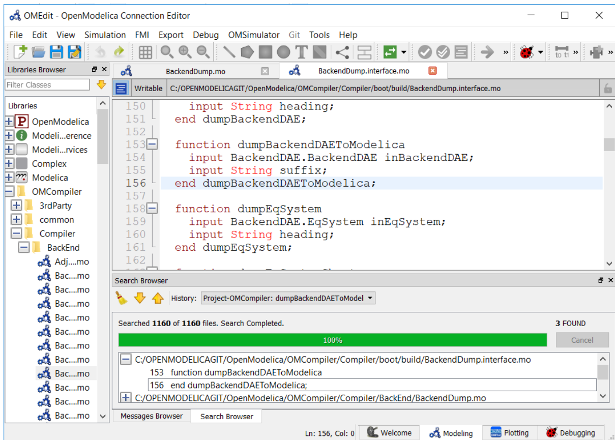
Figure 2.20: Search Results
