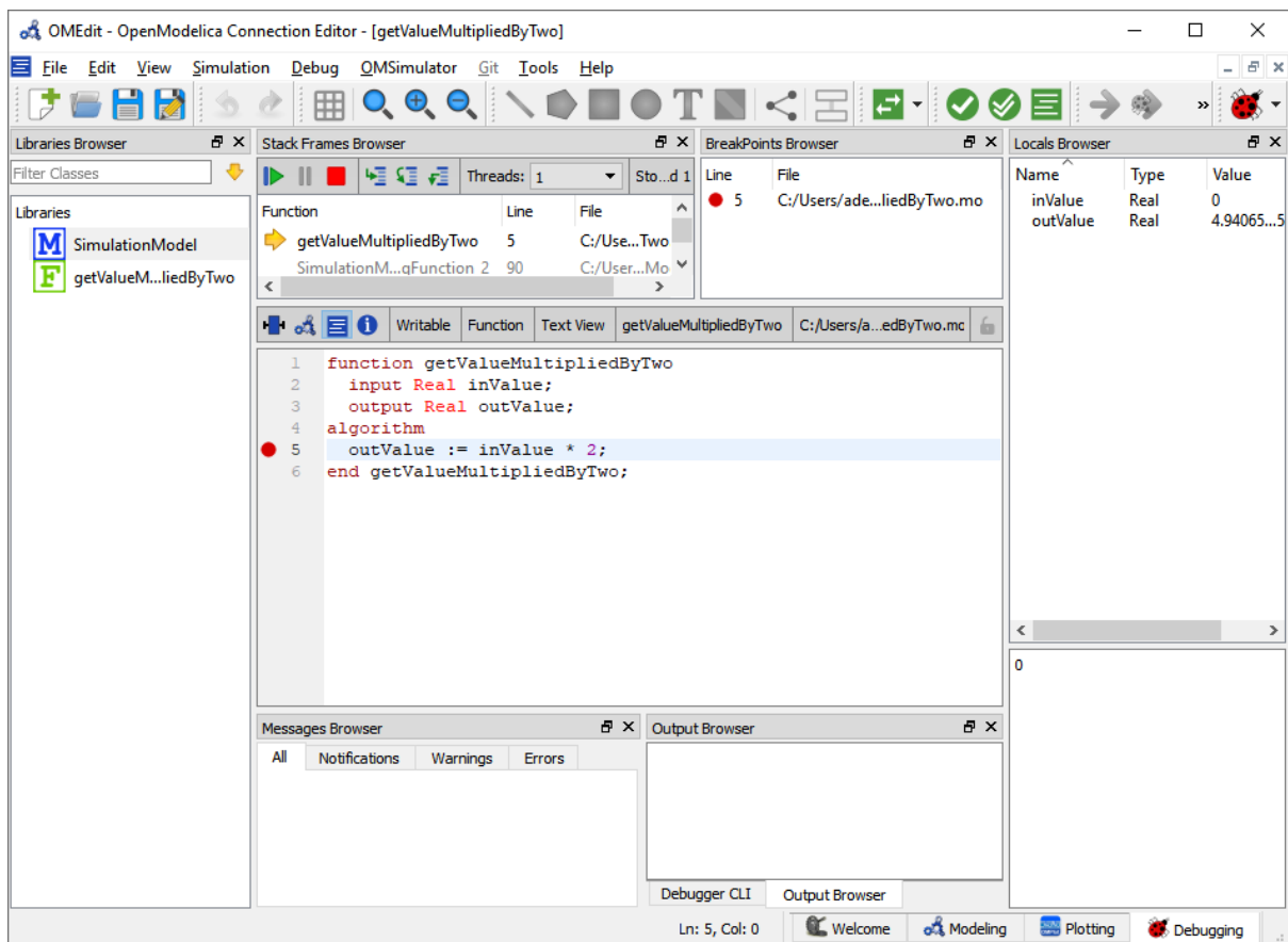
Figure 5.6: Algorithmic Debugger.
