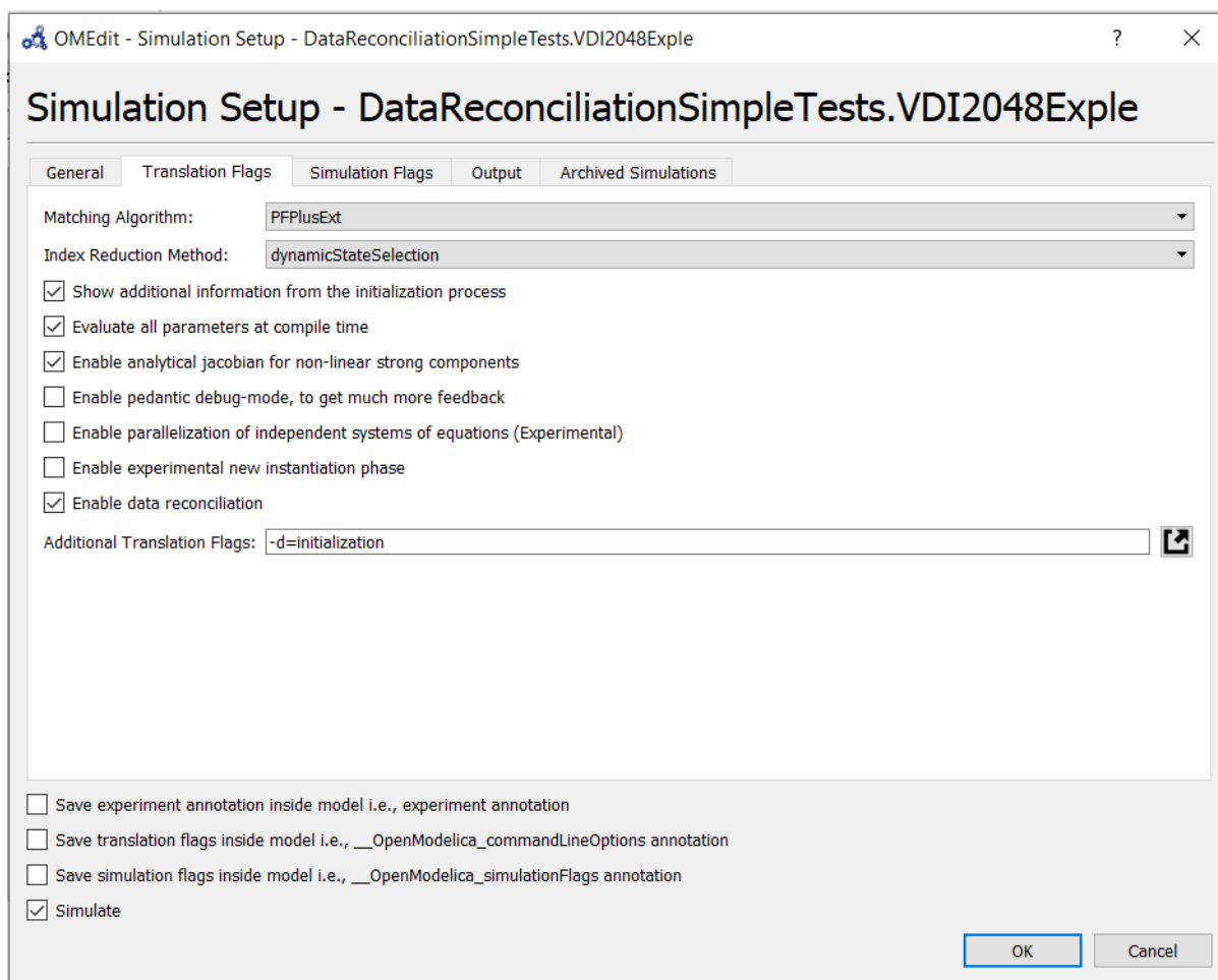
Figure 27.2: Setting DataReconciliation TraslationFlag
