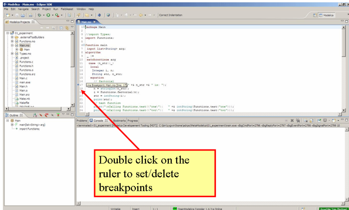
Figure 15.4: Setting/deleting breakpoints.
