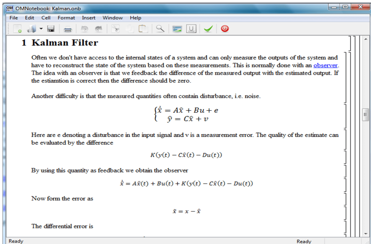
Figure 10.12: Theory background about Kalman filter.
