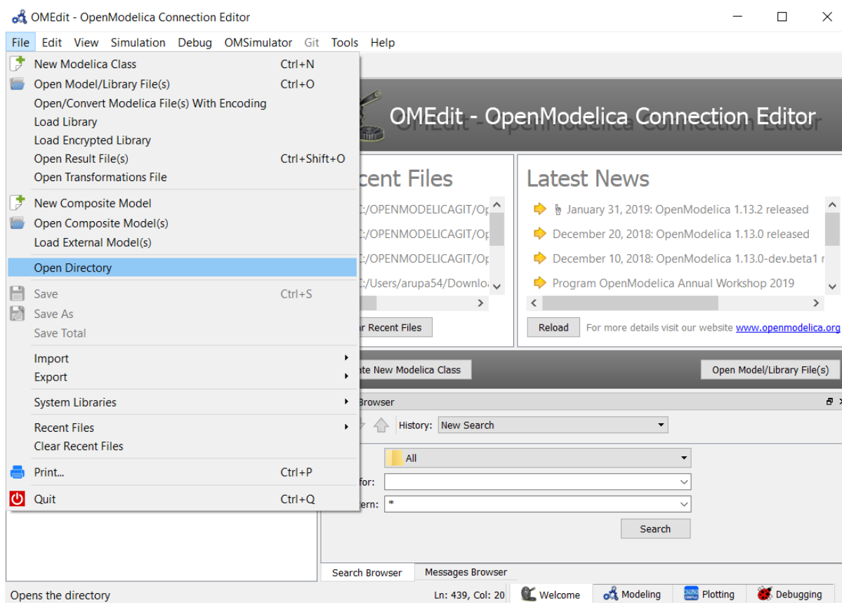
Figure 2.16: open-directory
