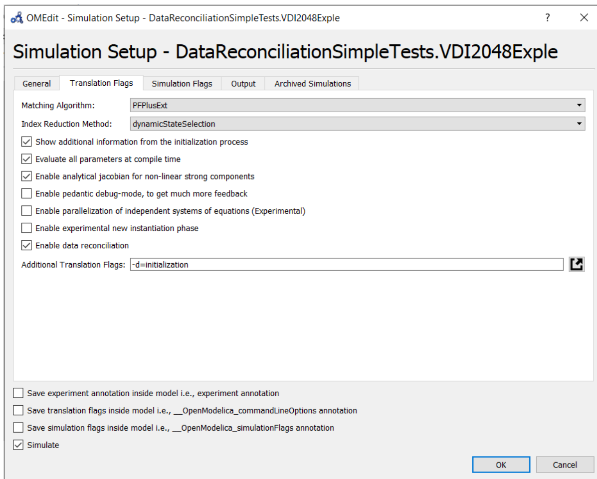
Figure 27.2: Setting DataReconciliation TranslationFlag
