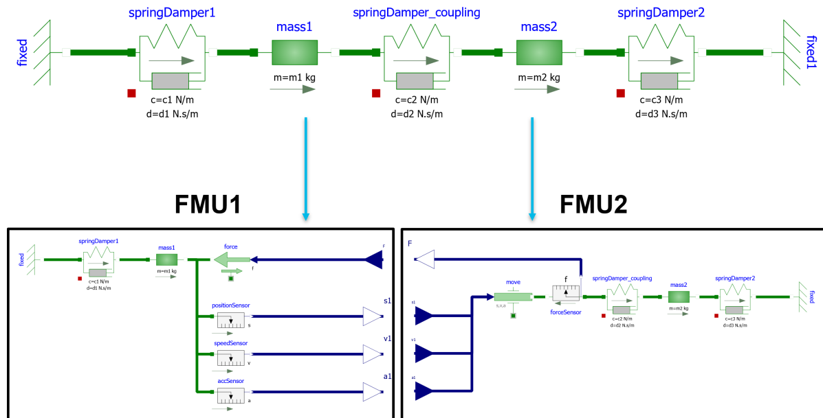
Figure 14.16: Dual mass oscillator Modelica model (diagram view) and FMUs
