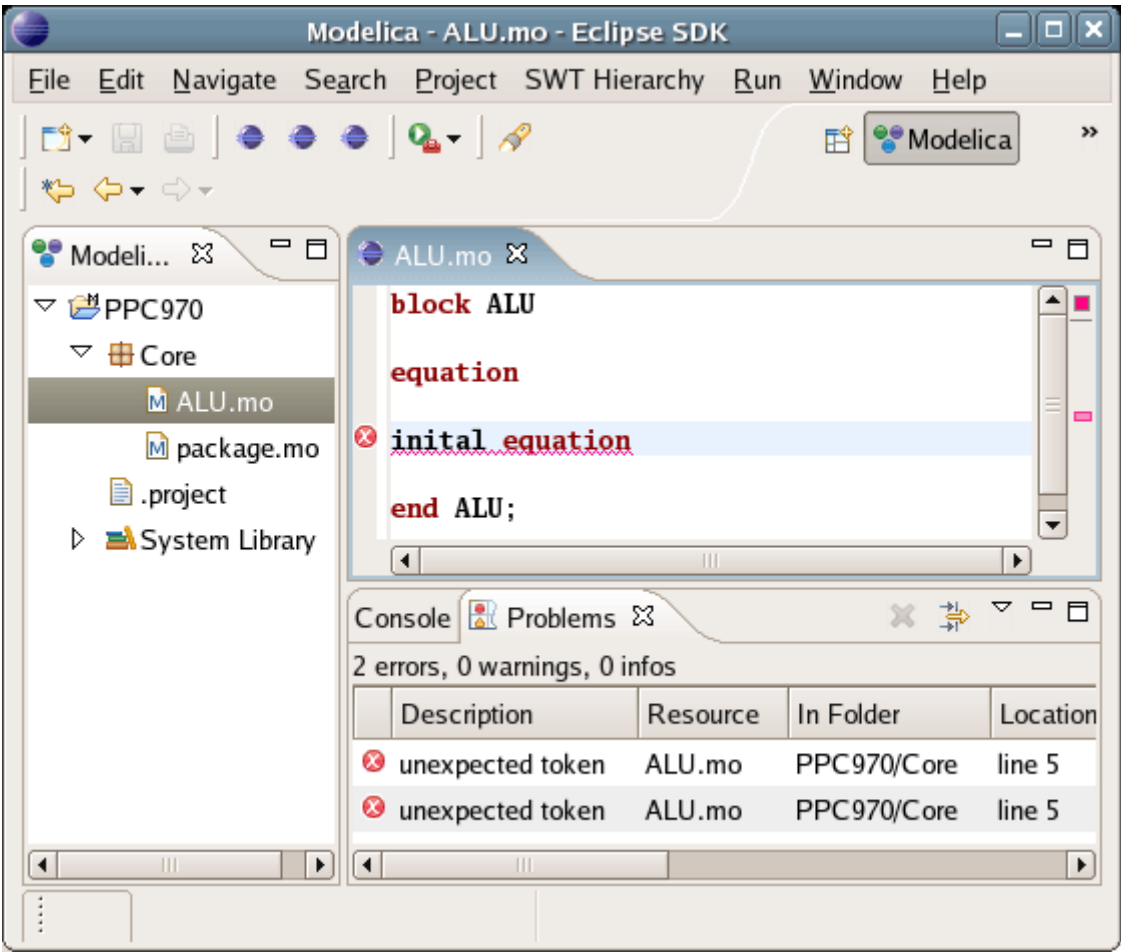
Figure 21.10: Syntax checking.
