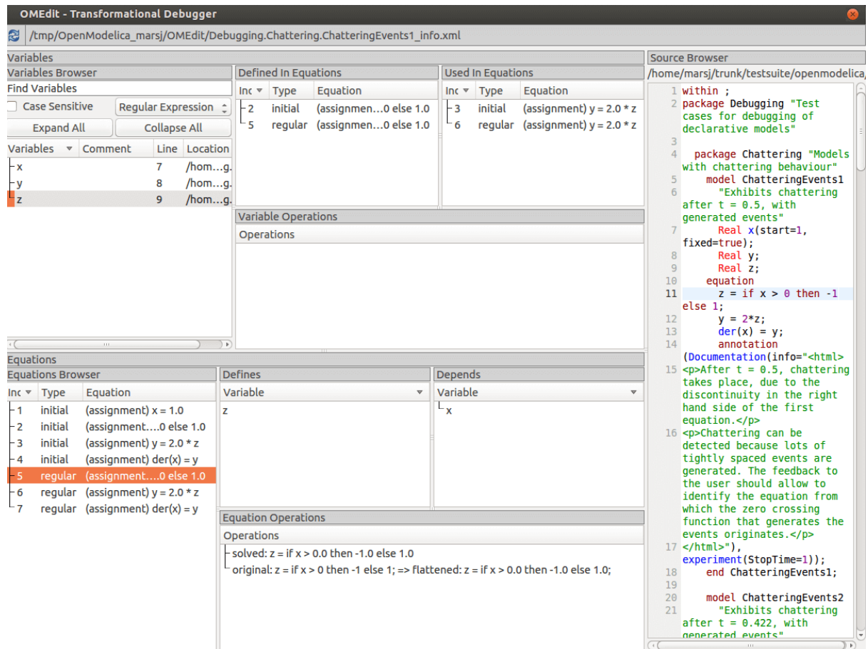
Figure 8.2: Transformations Browser.
