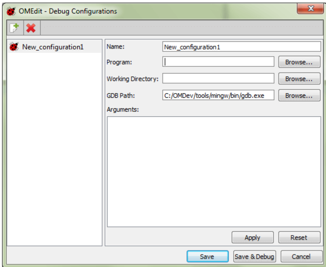
Figure 7.4: Debug Configurations.
