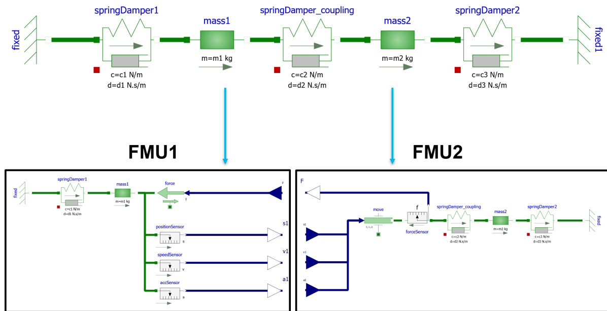
Figure 12.11: Dual mass oscillator Modelica model (diagram view) and FMUs
