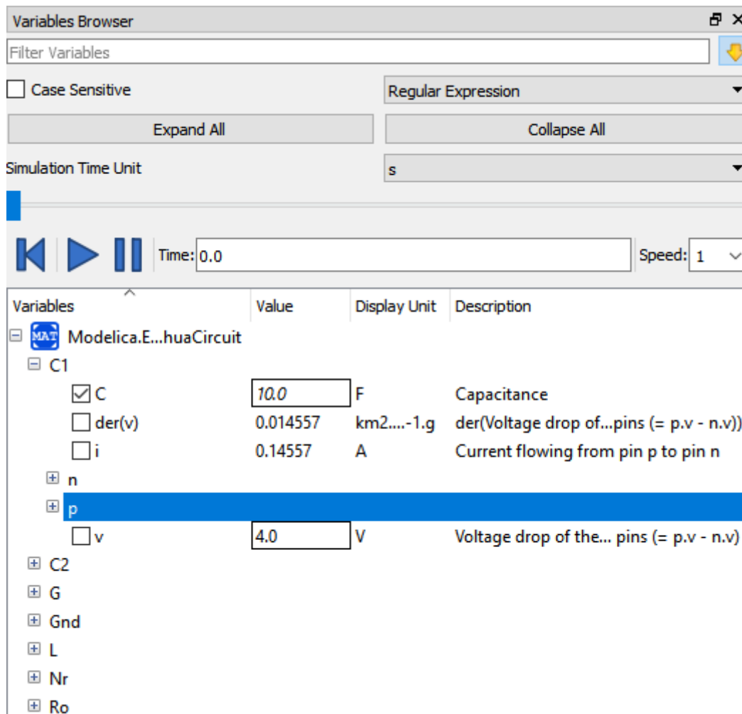
Figure 3.4: Variables Browser.
