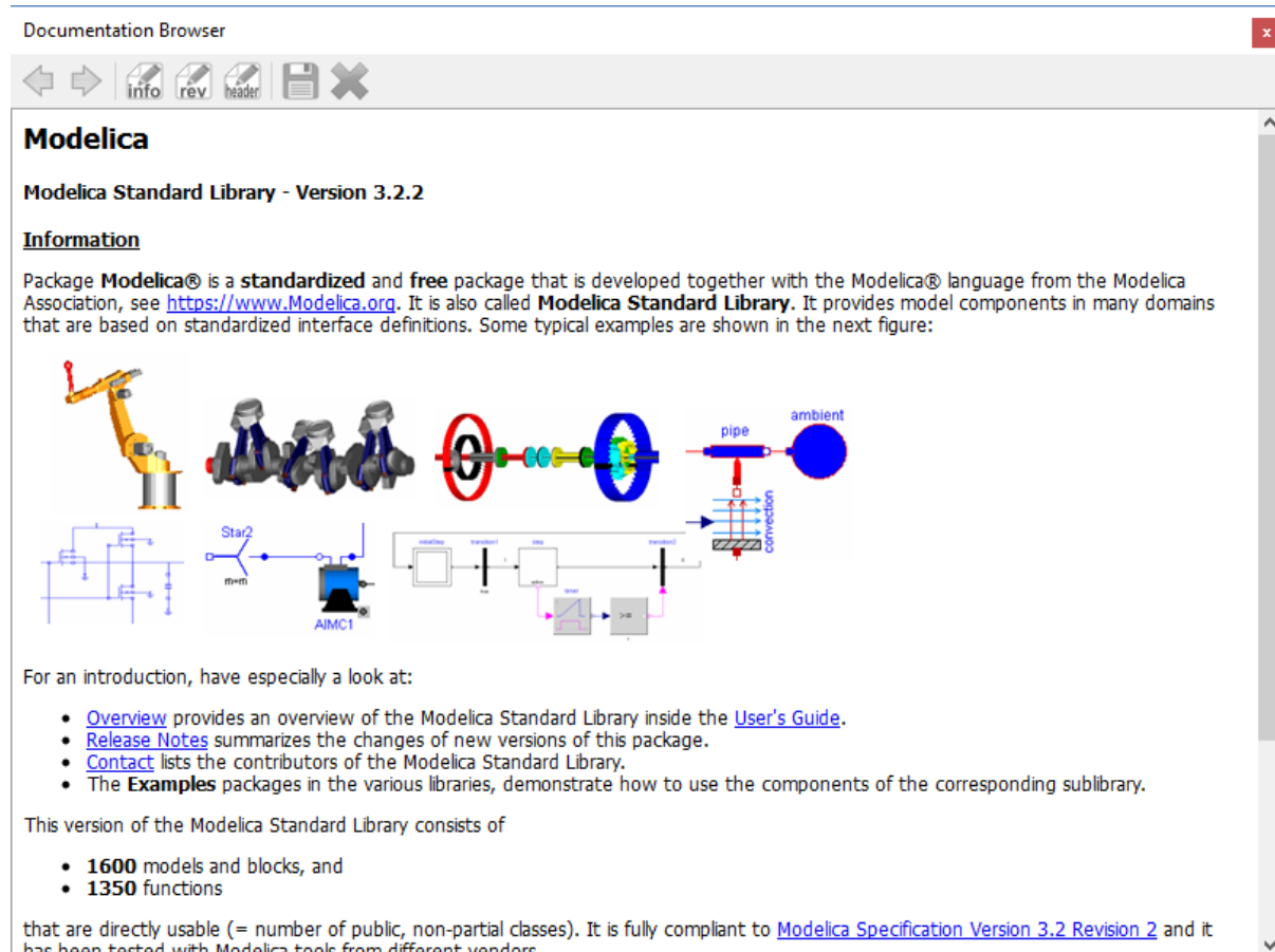
Figure 3.3: Documentation Browser.
