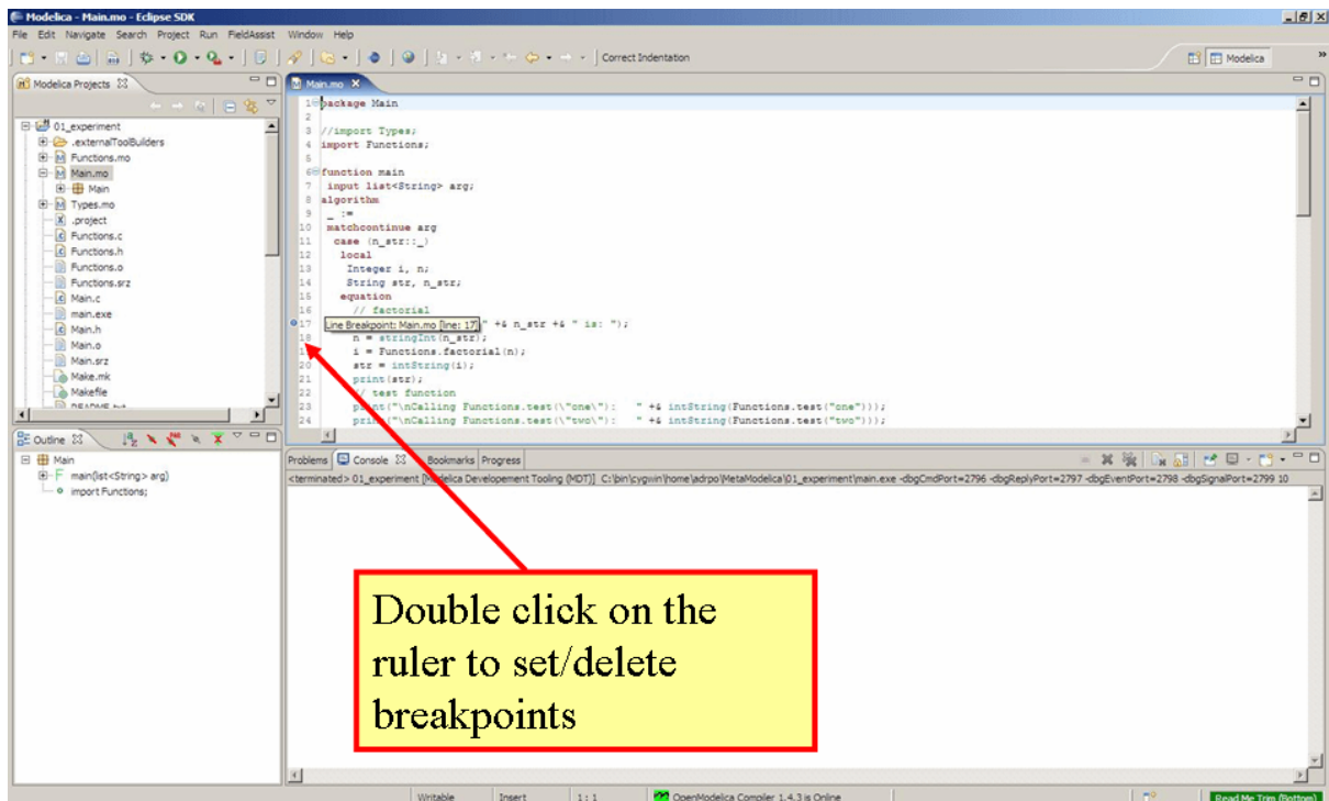
Figure 20.4: Setting/deleting breakpoints.
