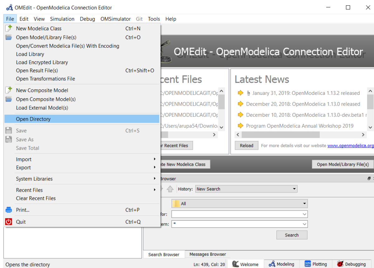
Figure 3.18: open-directory
