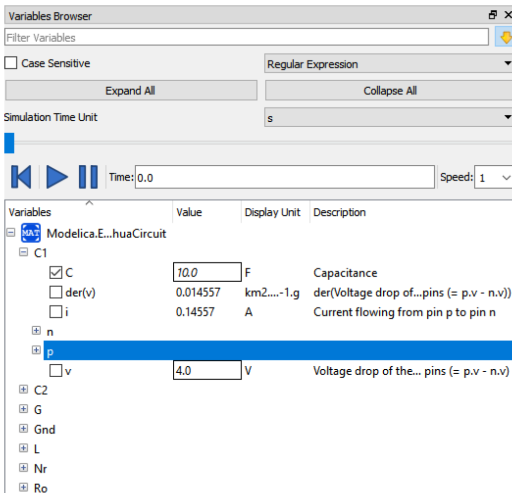
Figure 3.4: Variables Browser.
