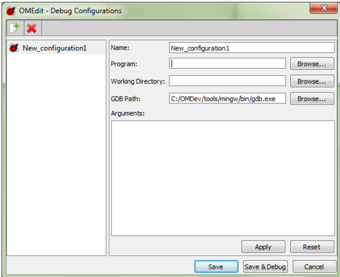
Figure 7.4: Debug Configurations.
