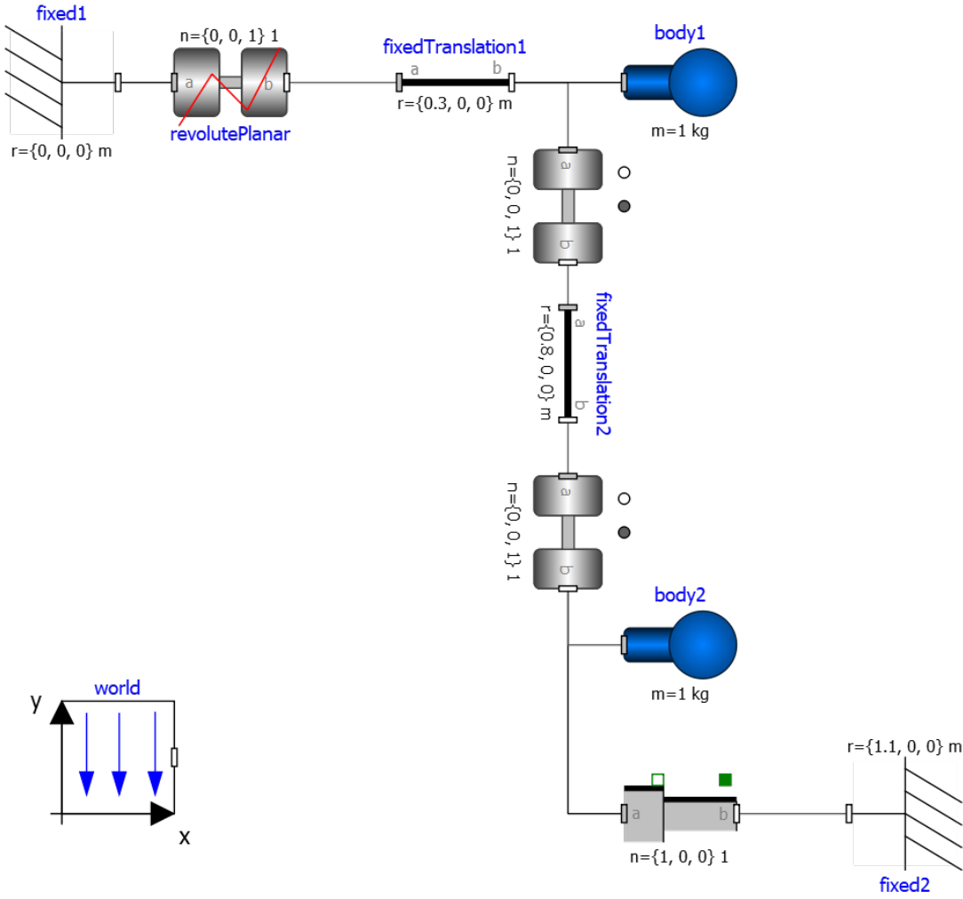
Figure 6.1: piston.mo
