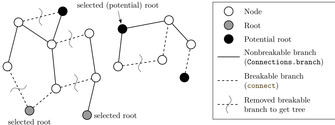
Figure 9.2: Example of a virtual connection graph.
