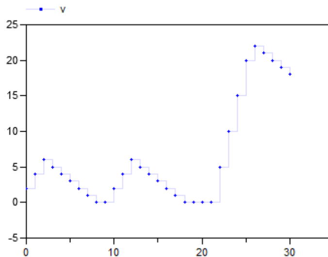
Figure 17.2: State machine behavior, as reflected by the variable v .
