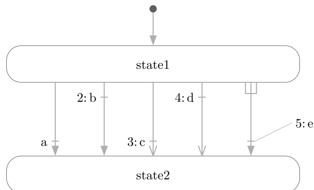
Figure 17.1: Recommended layout of a simple state machine. For the 5 transitions, the settings are as follows, from left to right: immediate = true, false, true, false, true ; reset = true, true, false, false, true ; synchronize = false, false, false, false, true ; priority = 1, 2, 3, 4, 5 .
